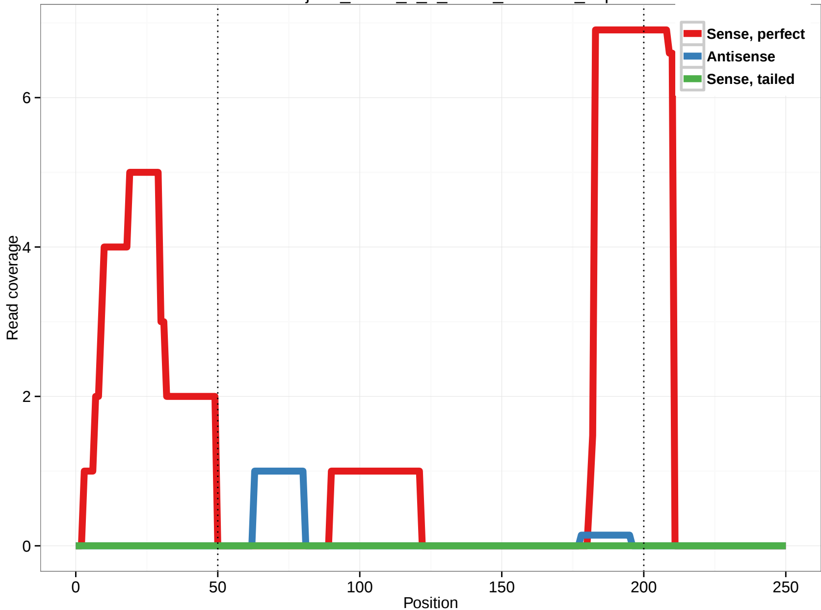
uc010xjm.1_intron_7_0_chr19_7516153_f.5p
