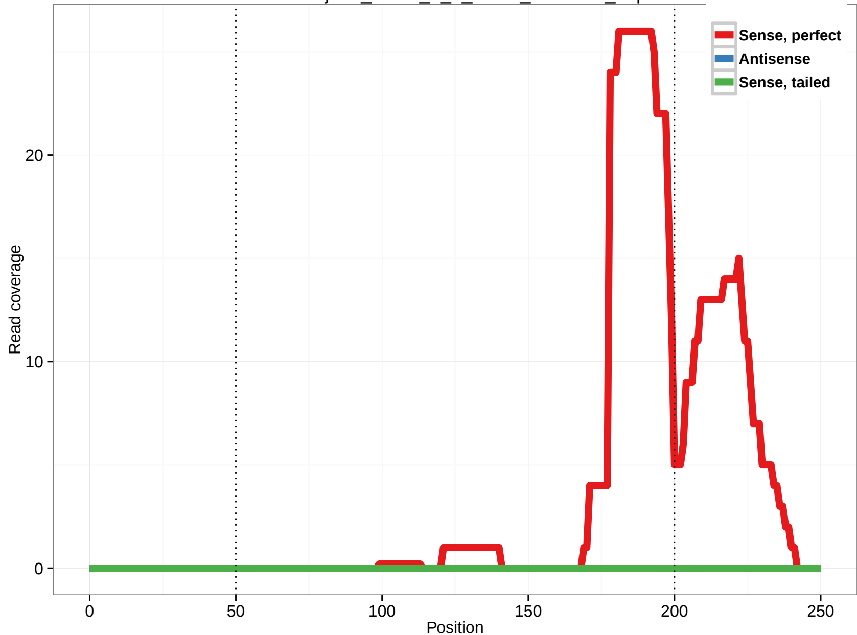
uc010xjm.1_intron_7_0_chr19_7516153_f.3p
