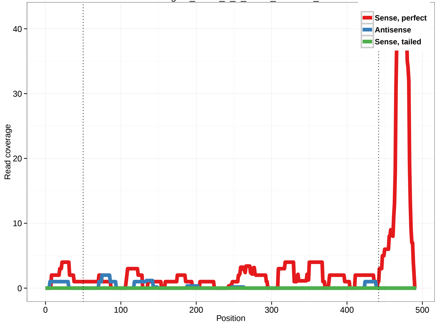
uc010xgu.1_intron_3_0_chr19_2042034_r
