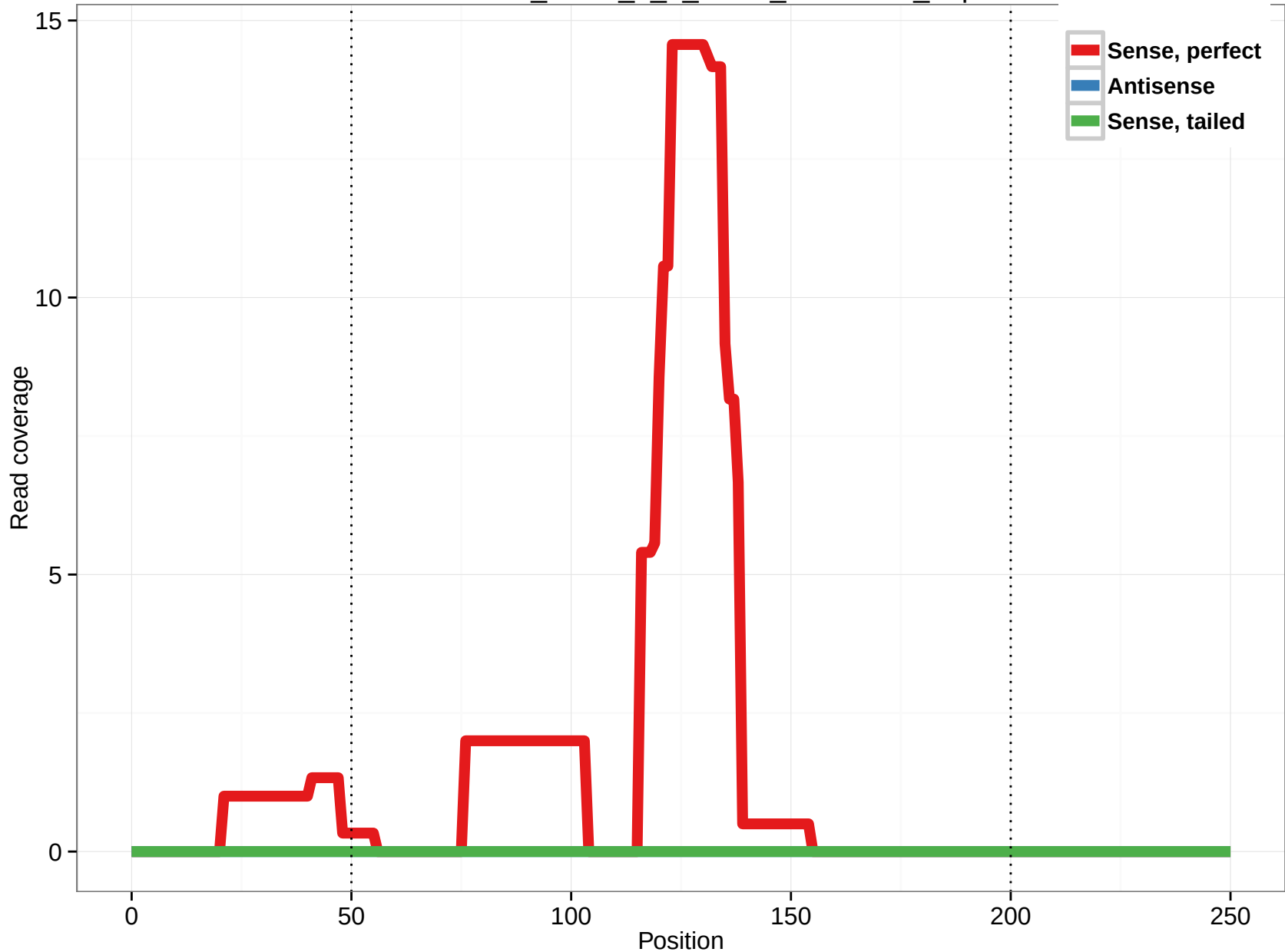
uc010xbk.1_intron_4_0_chr18_24209202_r.3p
