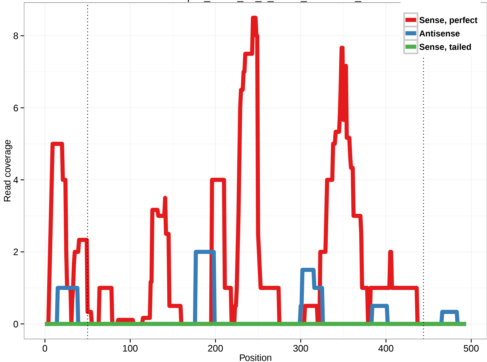
uc010wqc.1_intron_10_0_chr17_62777158_r
