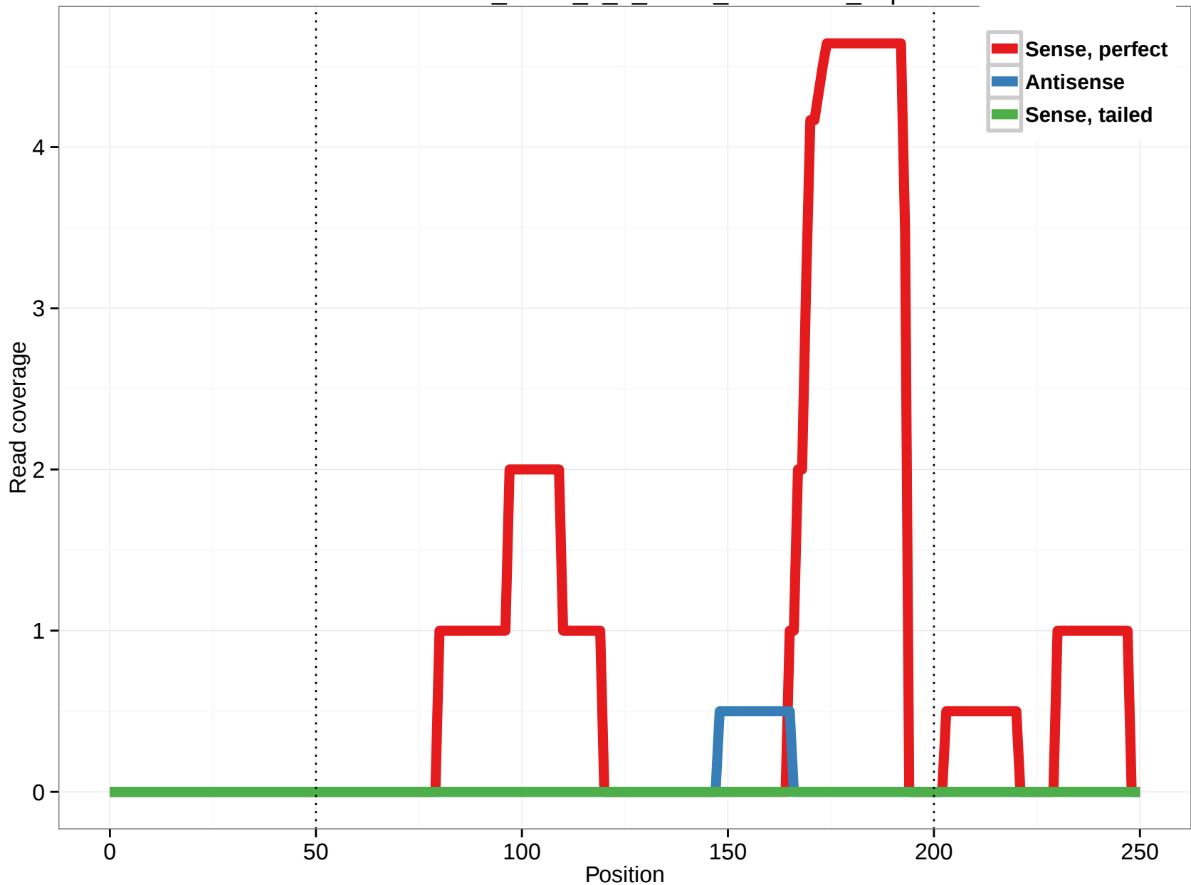
uc010wow.1_intron_0_0_chr17_58755276_f.3p
