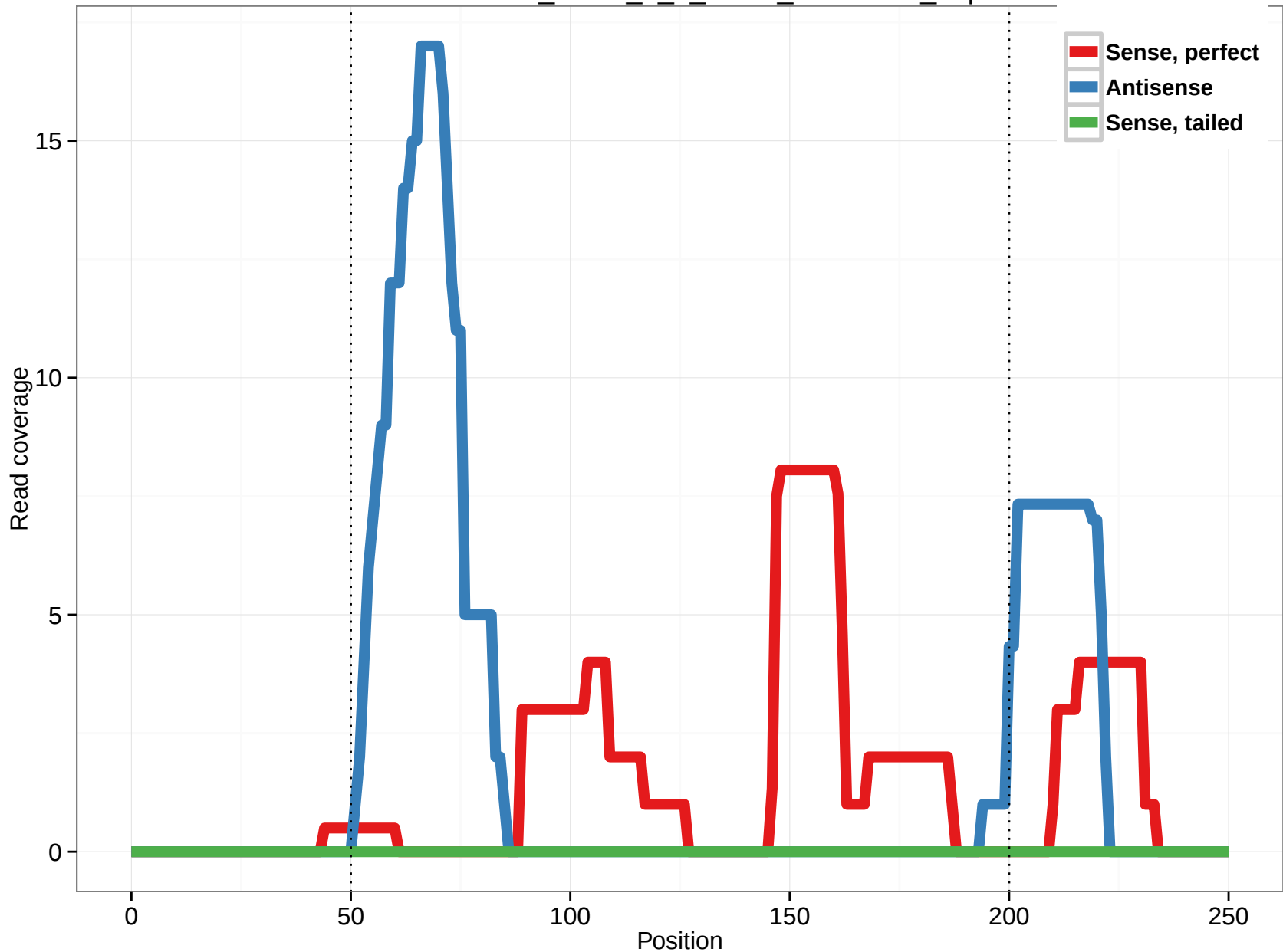
uc010wnm.1_intron_0_0_chr17_55333343_f.5p
