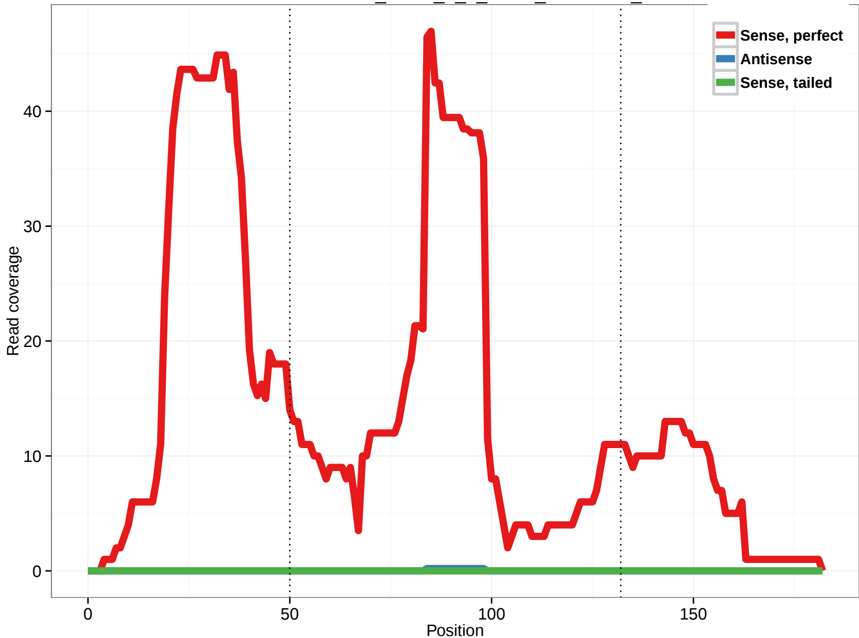
uc010wmw.1_intron_8_0_chr17_48828003_f
