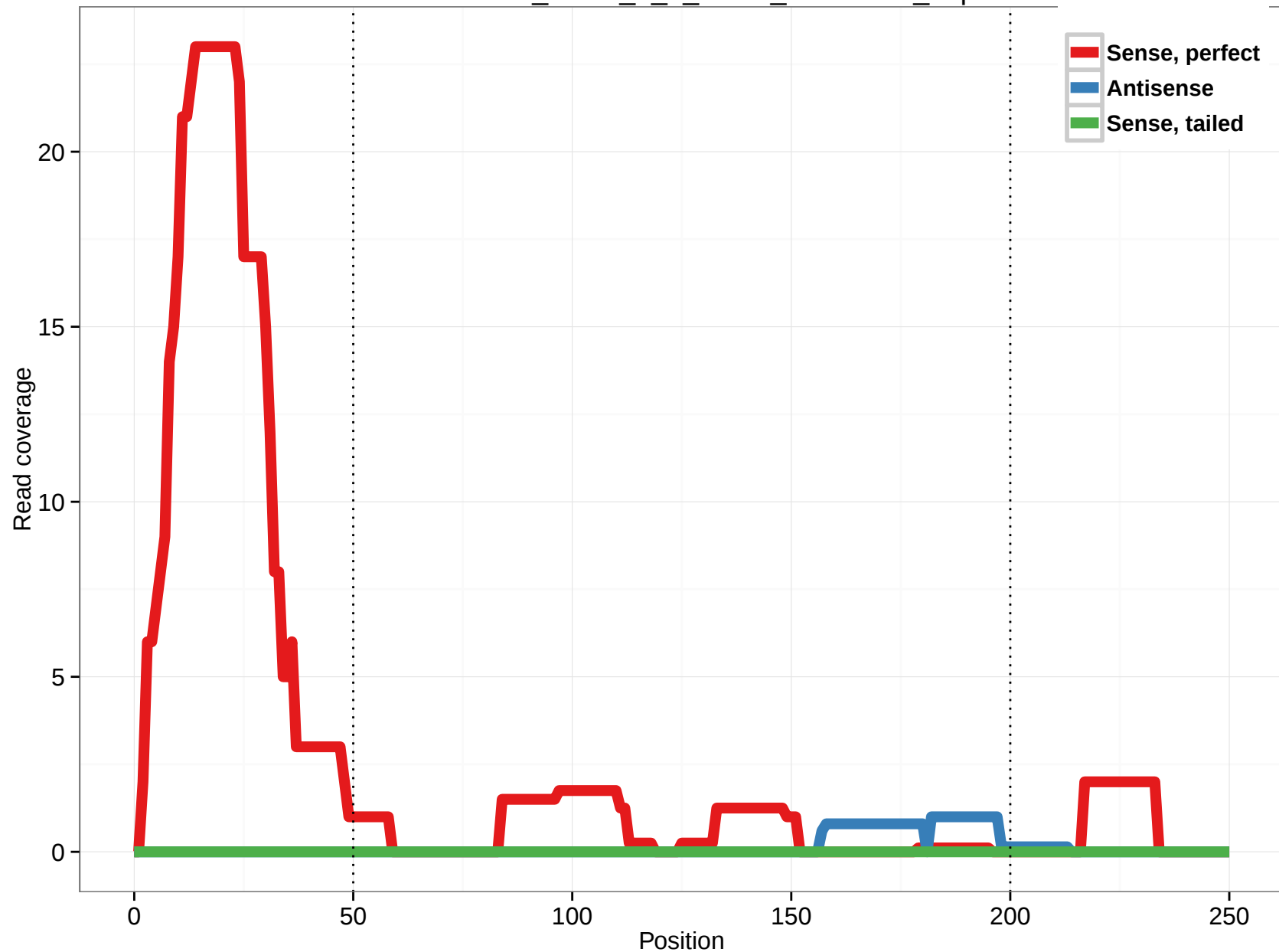
uc010wef.1_intron_6_0_chr17_37666015_f.5p
