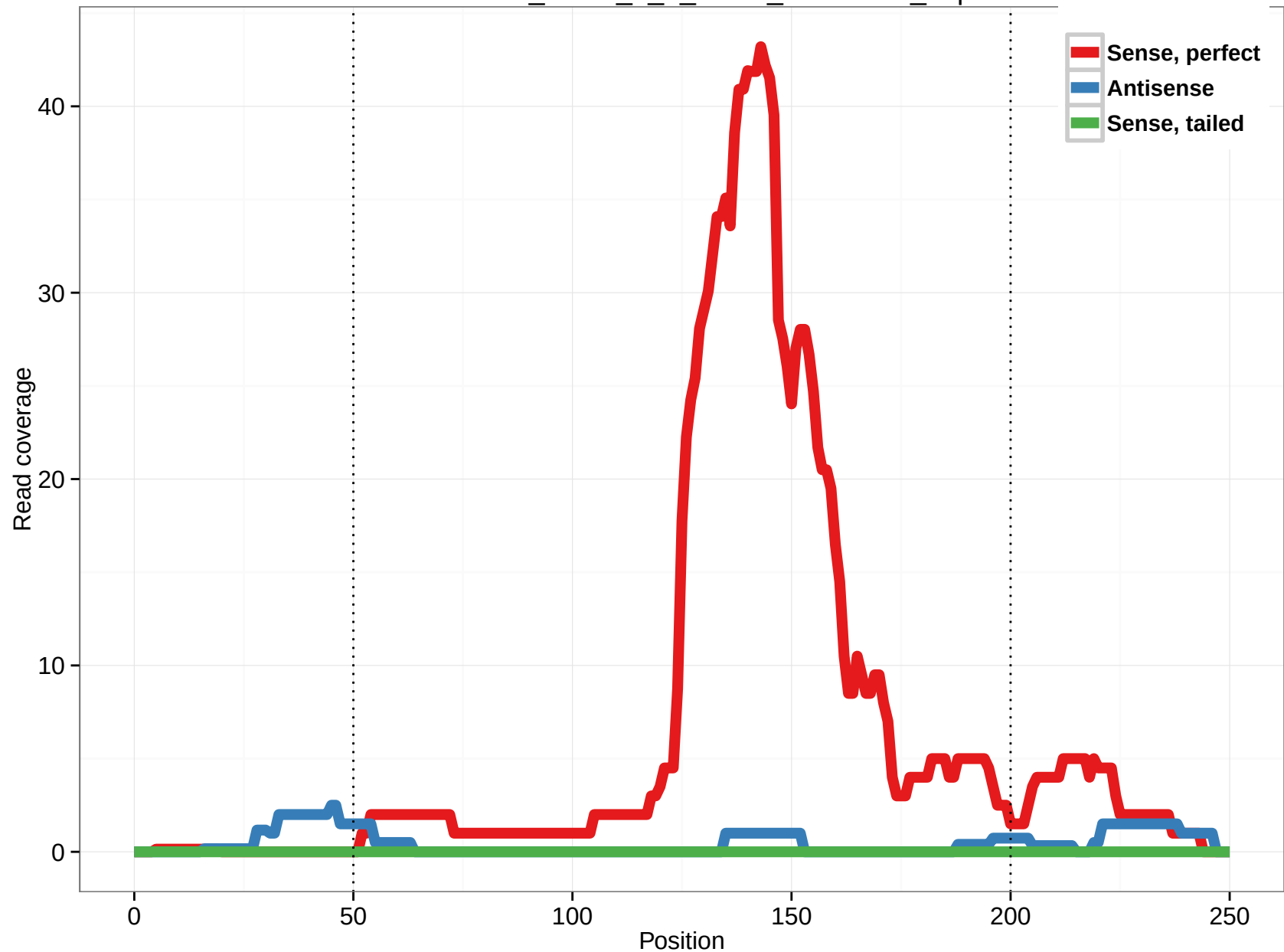
uc010vhl.1_intron_4_0_chr16_57284420_f.3p
