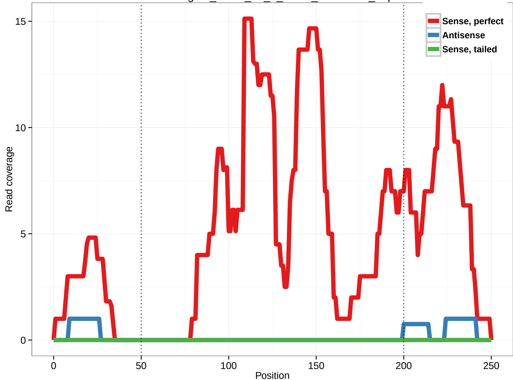
uc010vgh.1_intron_16_0_chr16_47493087_r.5p
