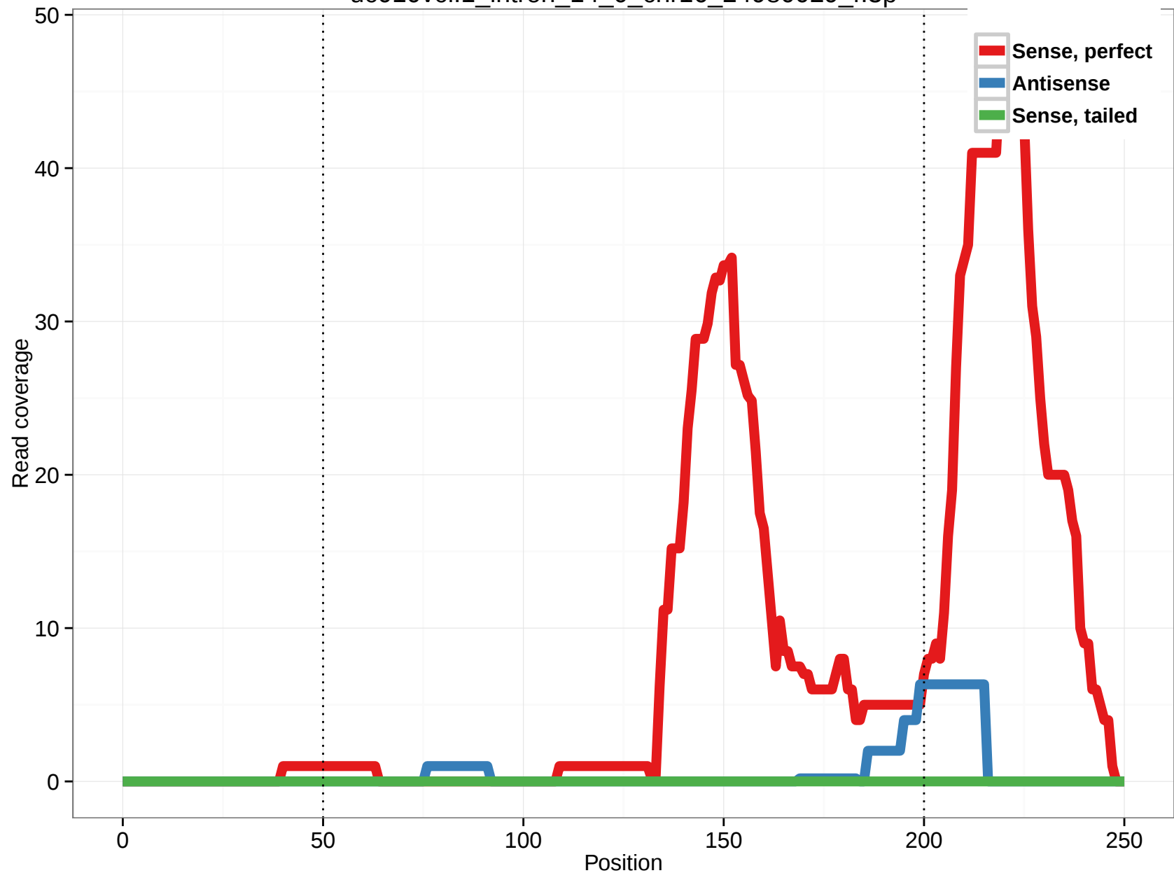
uc010vcf.1_intron_14_0_chr16_24980029_r.3p
