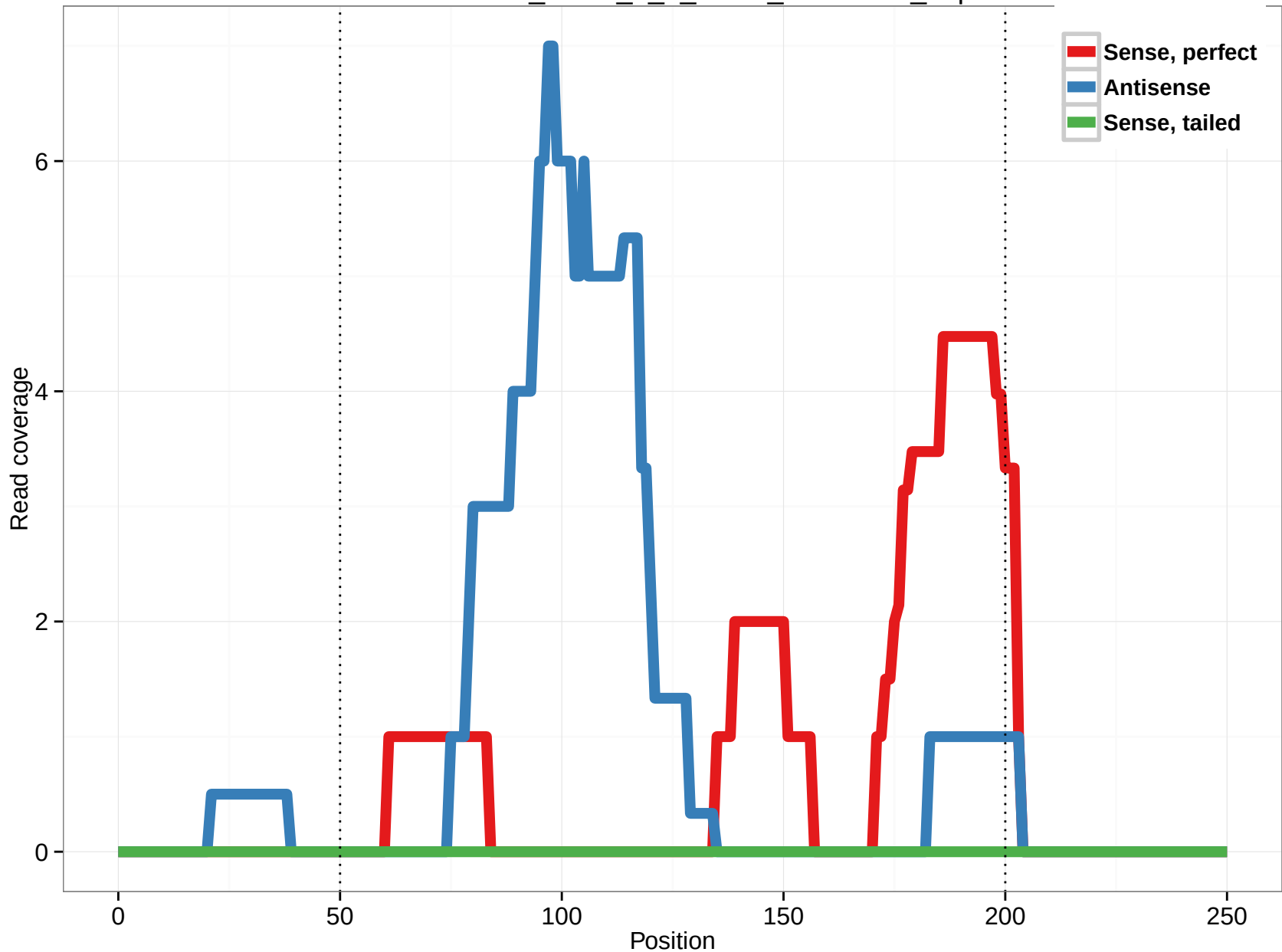
uc010umh.1_intron_7_0_chr15_75632562_f.3p
