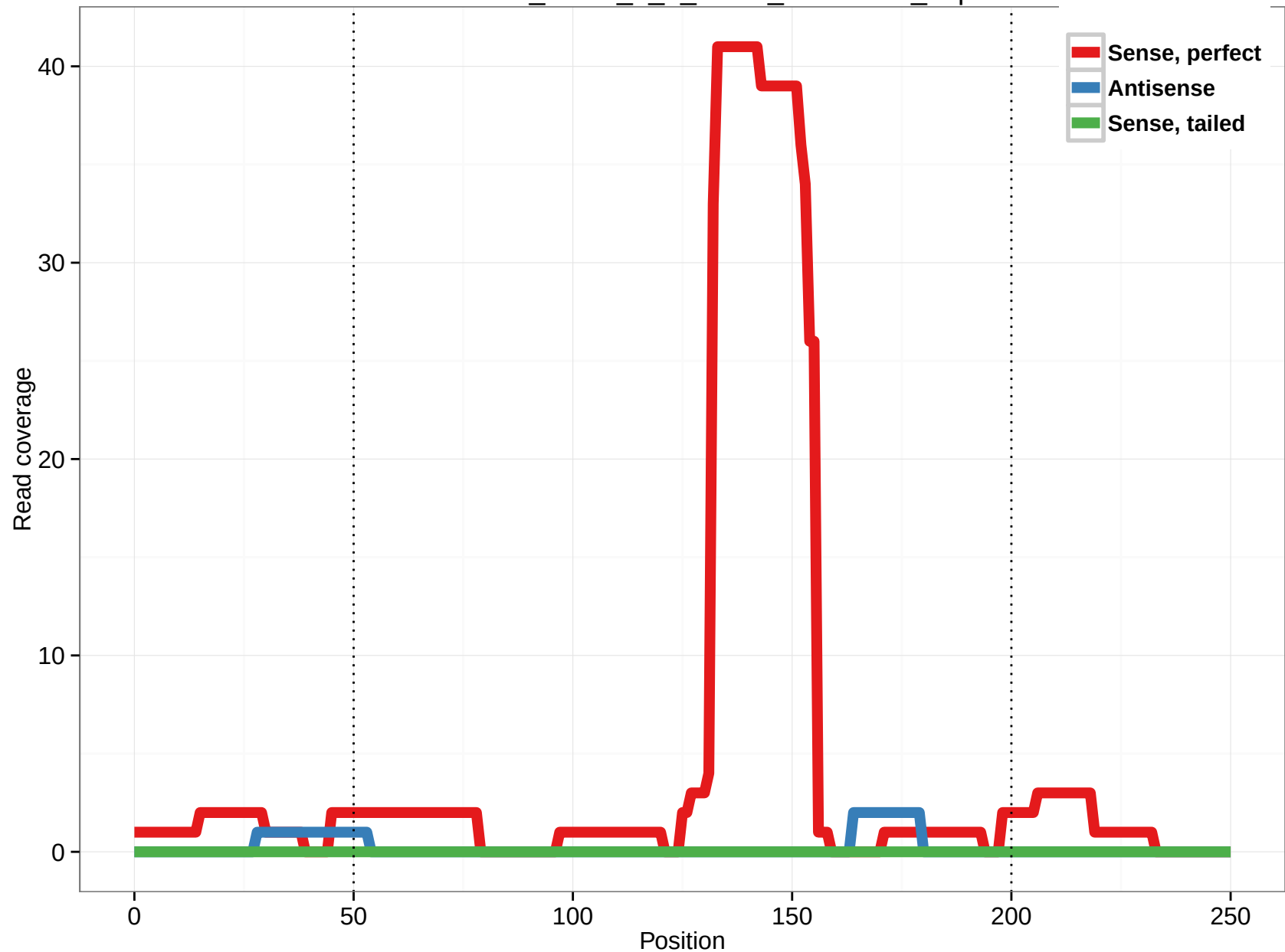
uc010ulv.1_intron_1_0_chr15_75182996_f.3p
