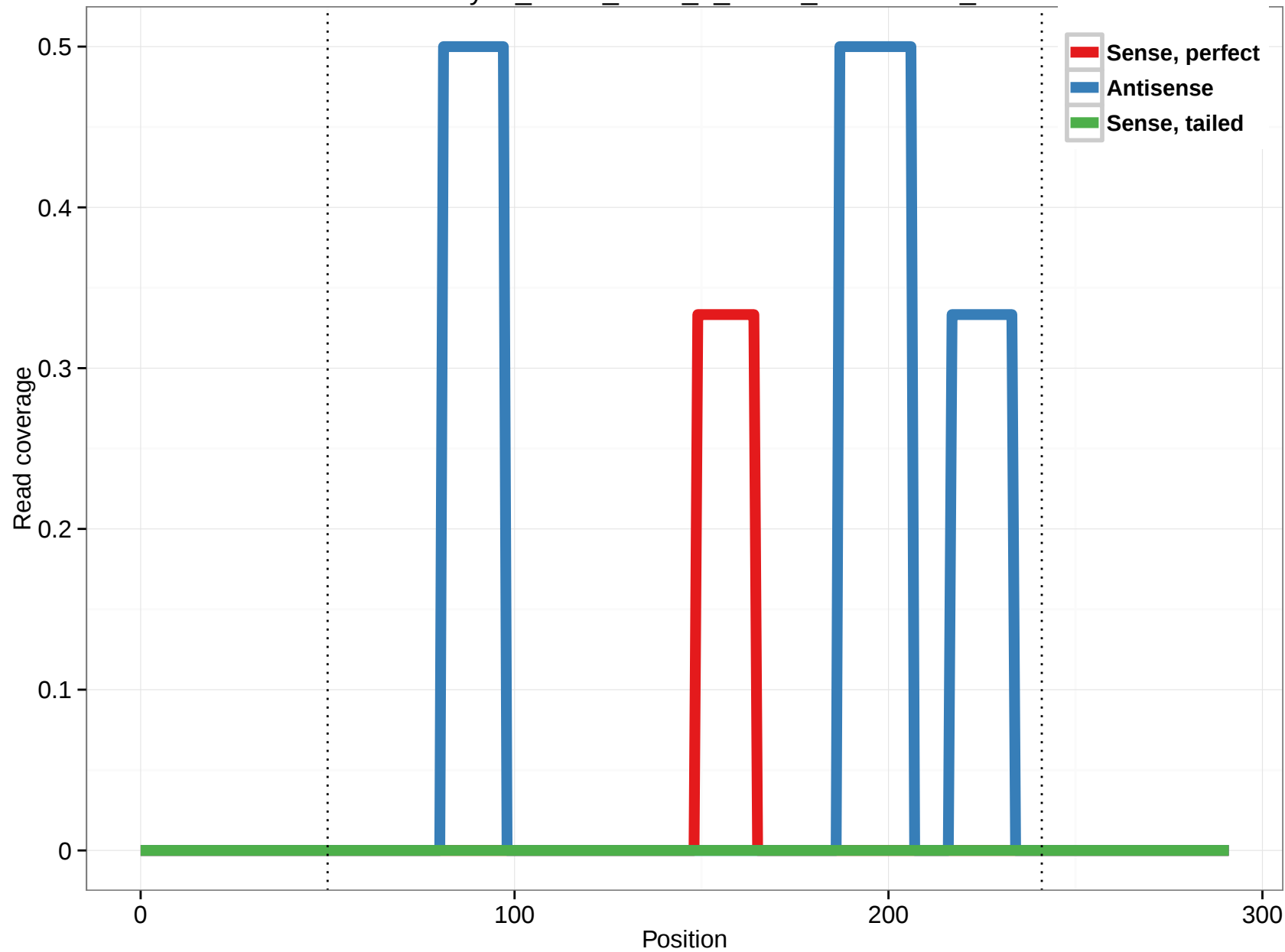
uc010tyt.1_intron_1975_0_chr14_106511197_r
