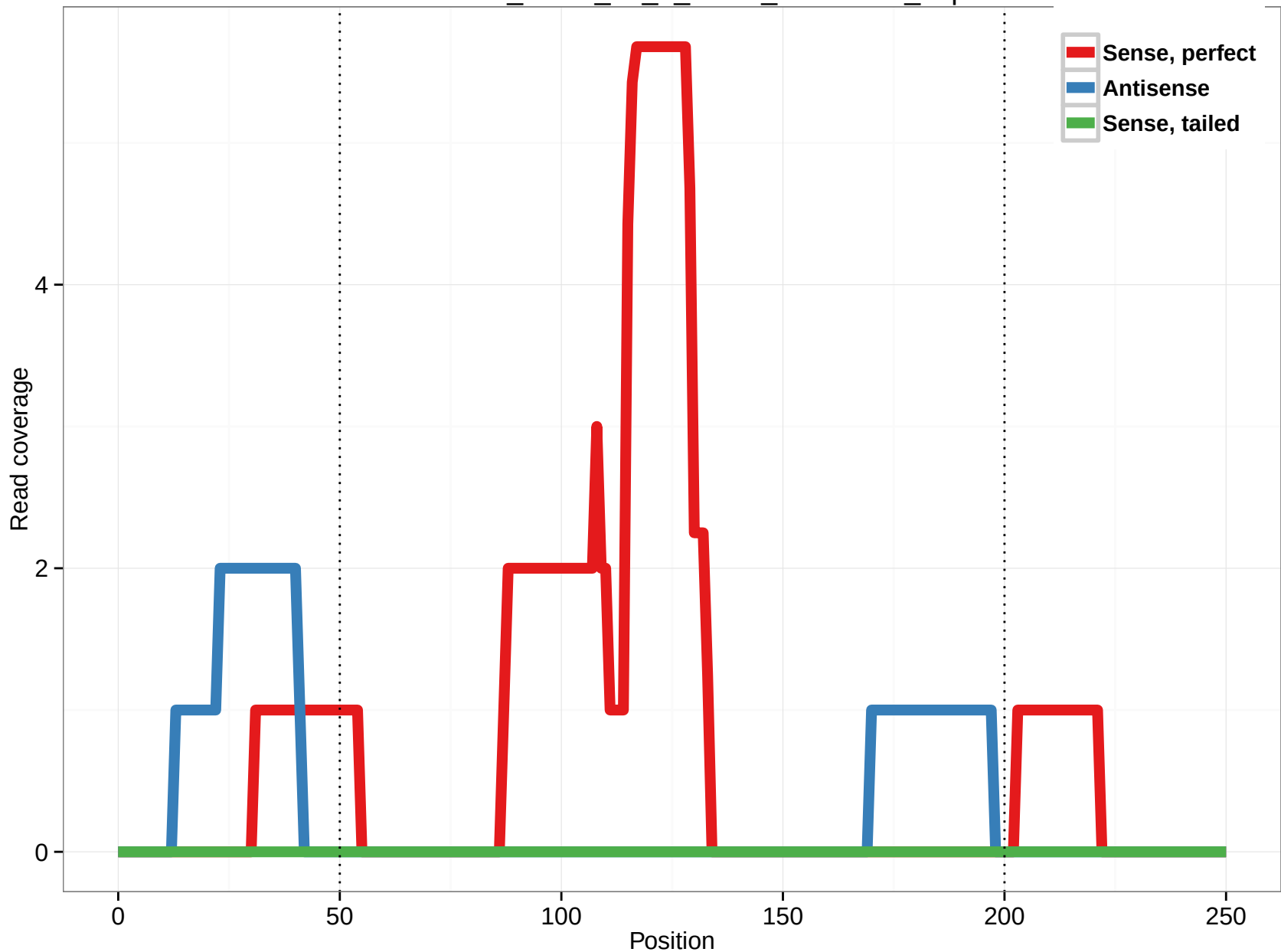
uc010tsl.1_intron_12_0_chr14_65521408_f.5p
