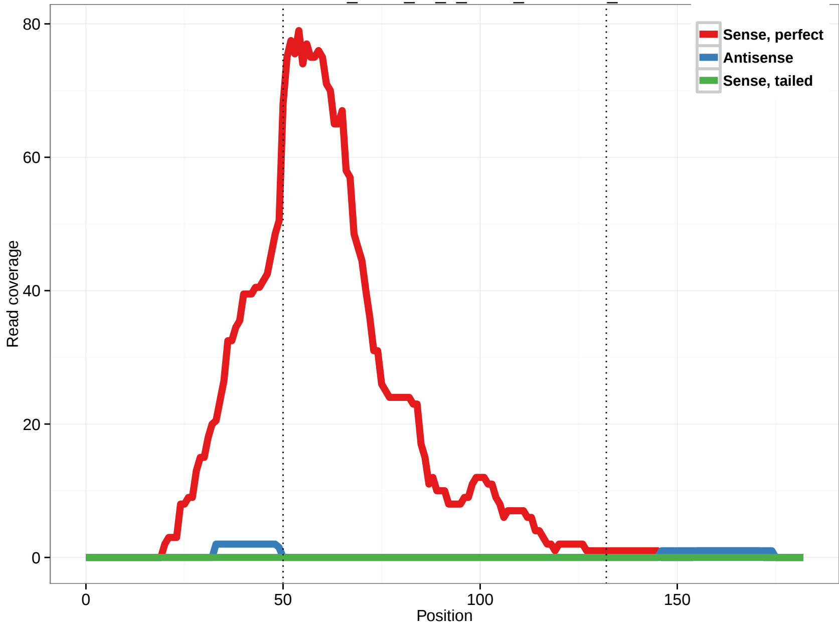
uc010tff.1_intron_10_0_chr13_41837621_r
