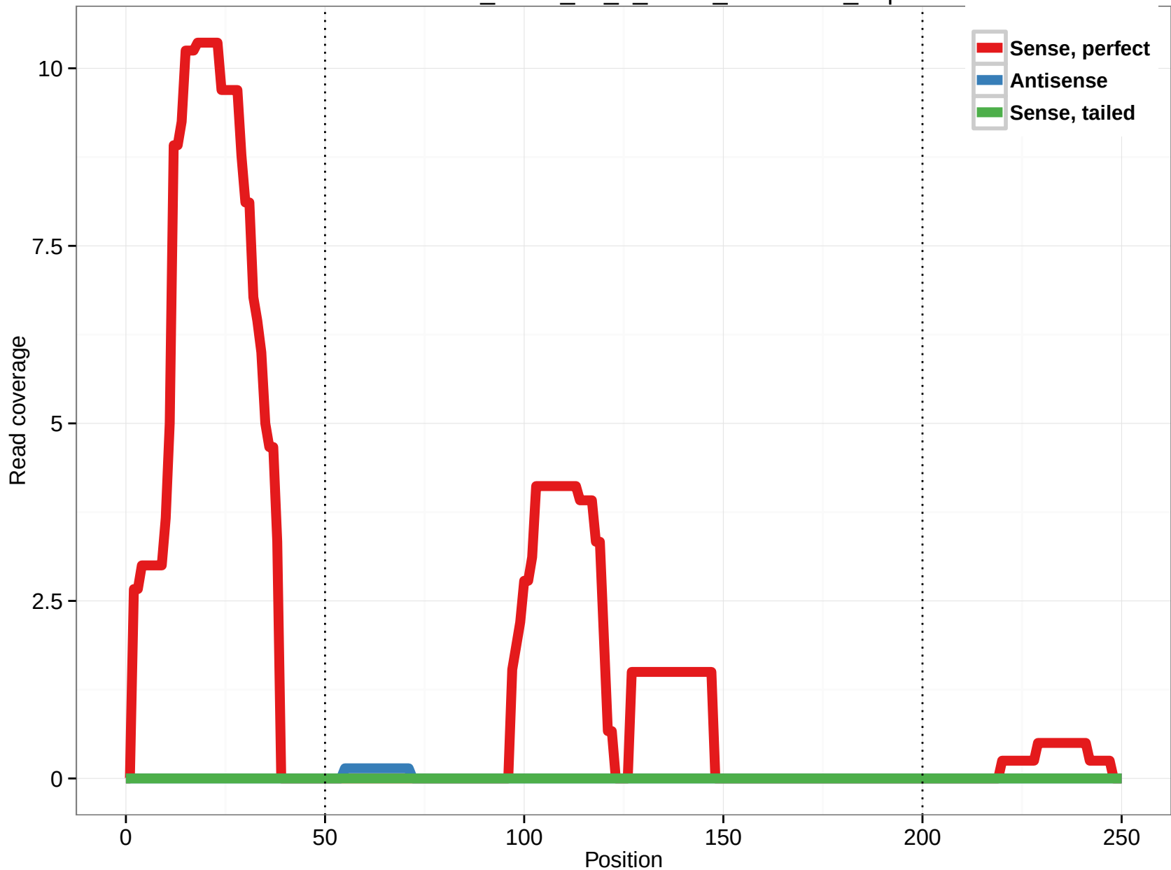
uc010tcm.1_intron_22_0_chr13_20133270_r.3p
