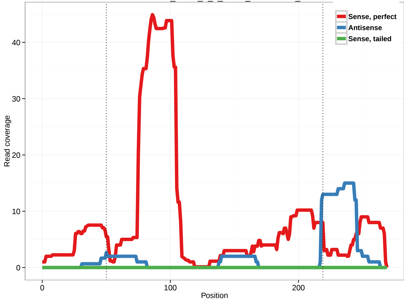
uc010tcd.1_intron_6_0_chr12_133780886_f
