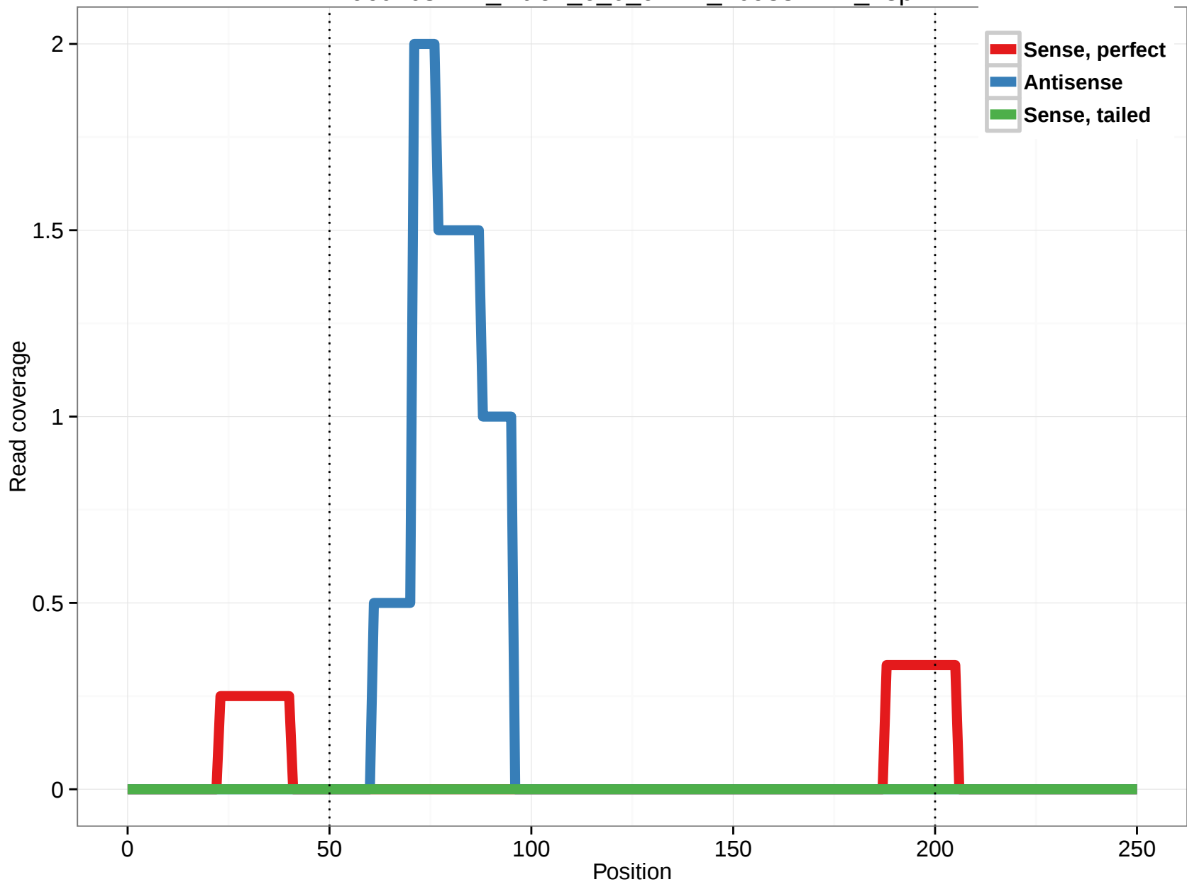
uc010sxh.1_intron_6_0_chr12_109331114_r.3p
