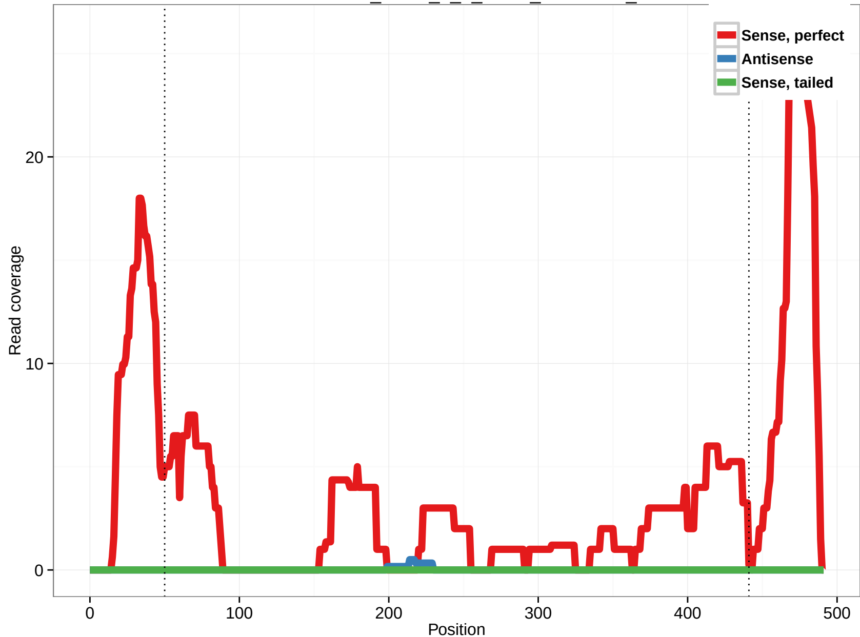
uc010soh.1_intron_5_0_chr12_53849278_f
