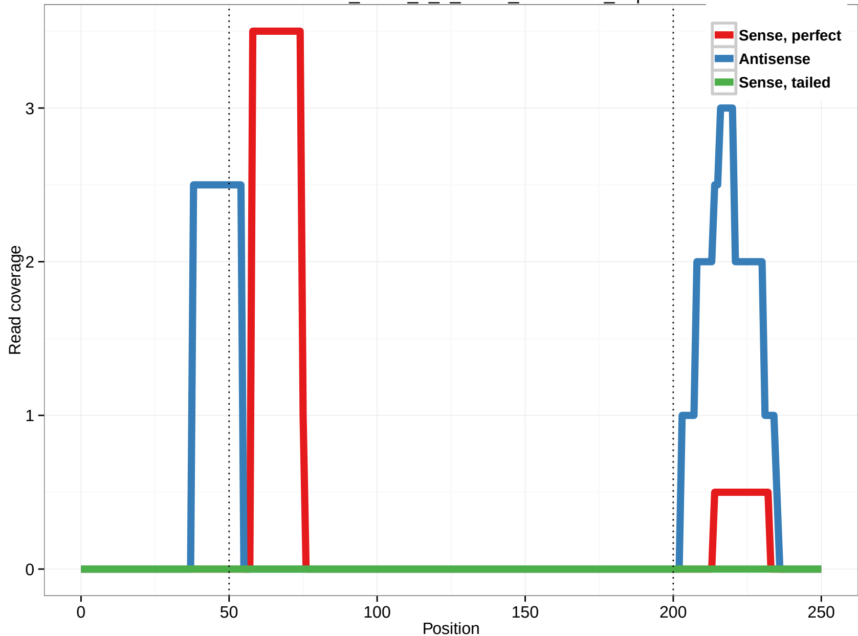
uc010snr.1_intron_4_0_chr12_52647550_r.3p
