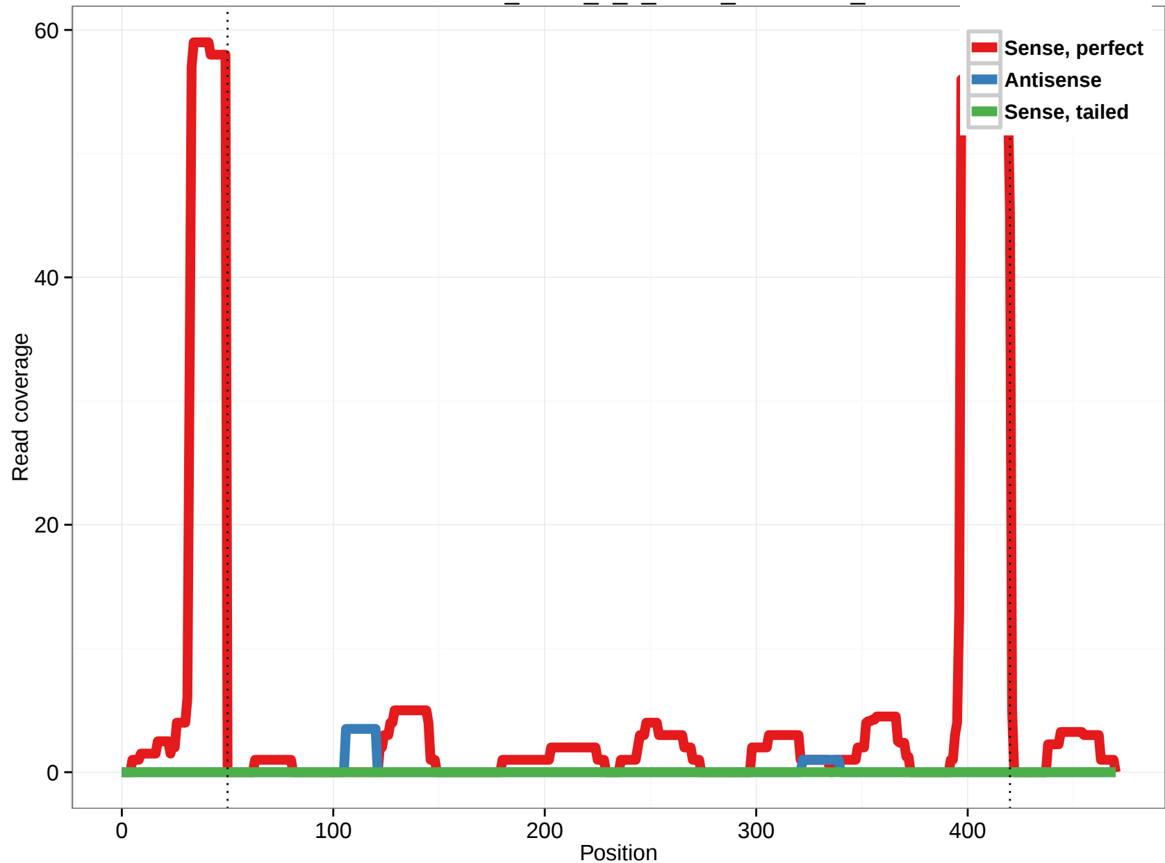
uc010sma.1_intron_1_0_chr12_49317636_r
