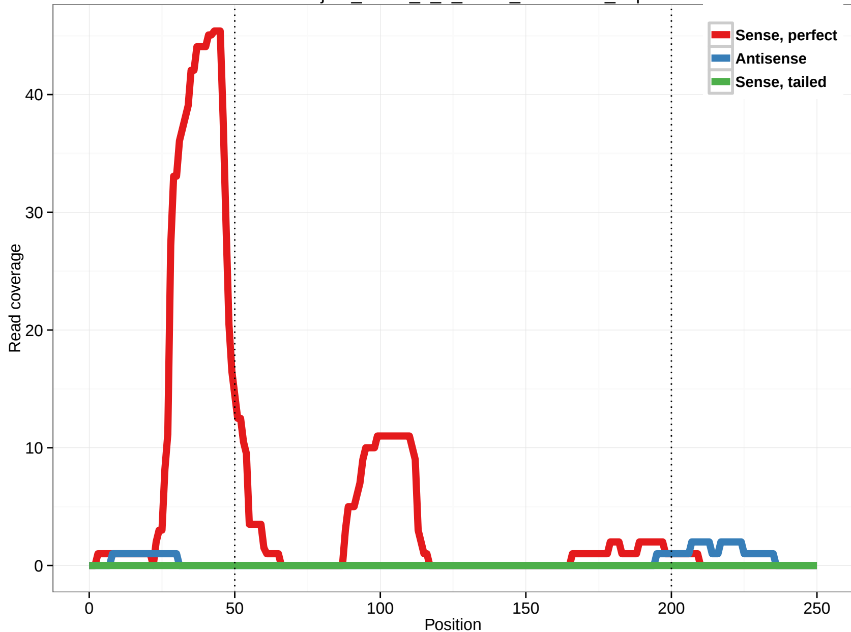
uc010sja.1_intron_0_0_chr12_25205891_f.5p
