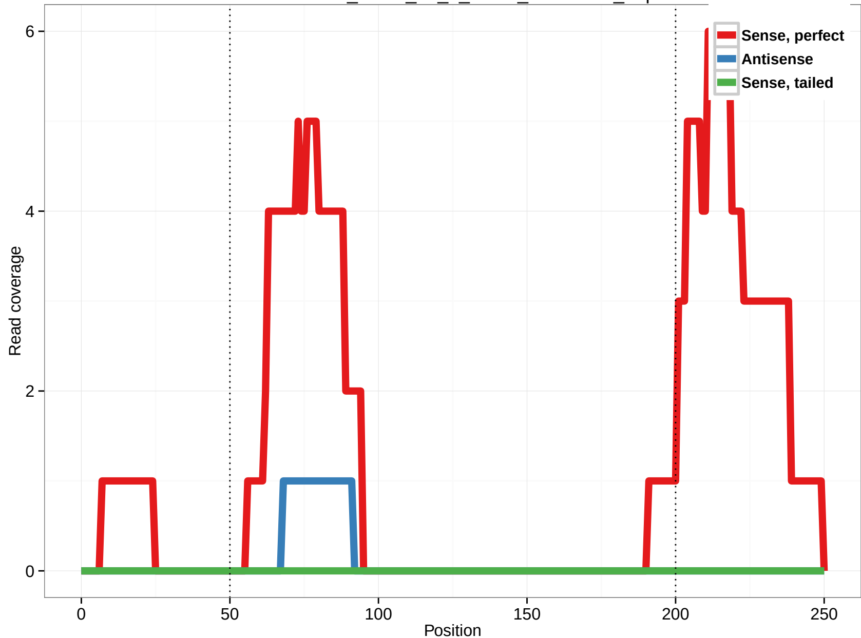
uc010shv.1_intron_10_0_chr12_15811520_r.3p
