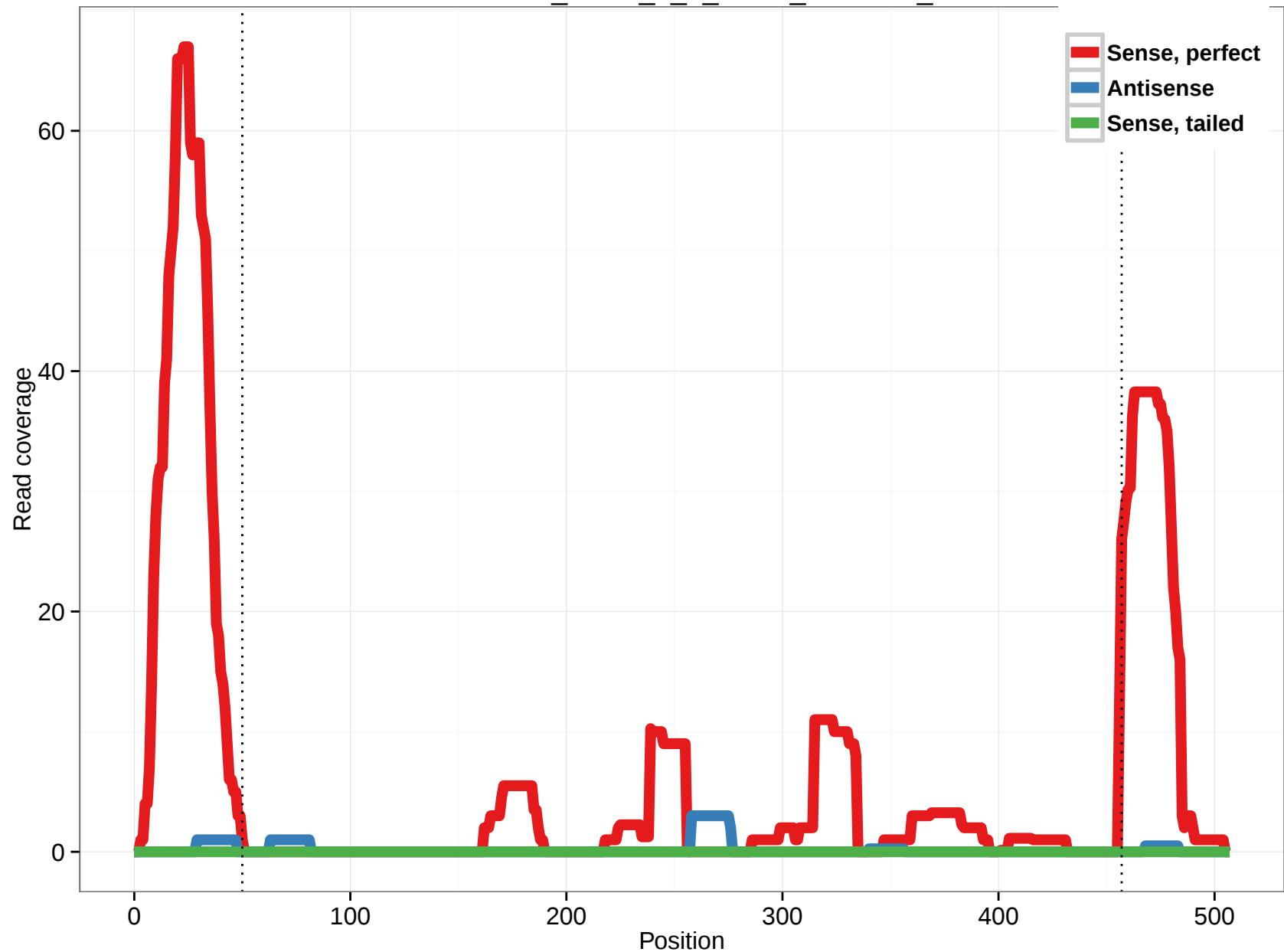
uc010sfi.1_intron_3_0_chr12_6859472_r
