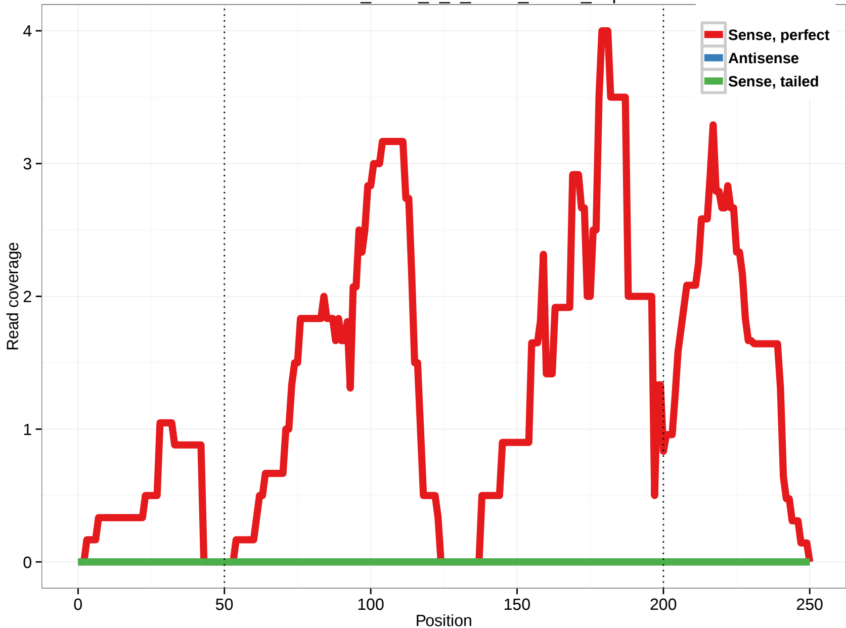
uc010scx.1_intron_0_0_chr12_74366_f.3p
