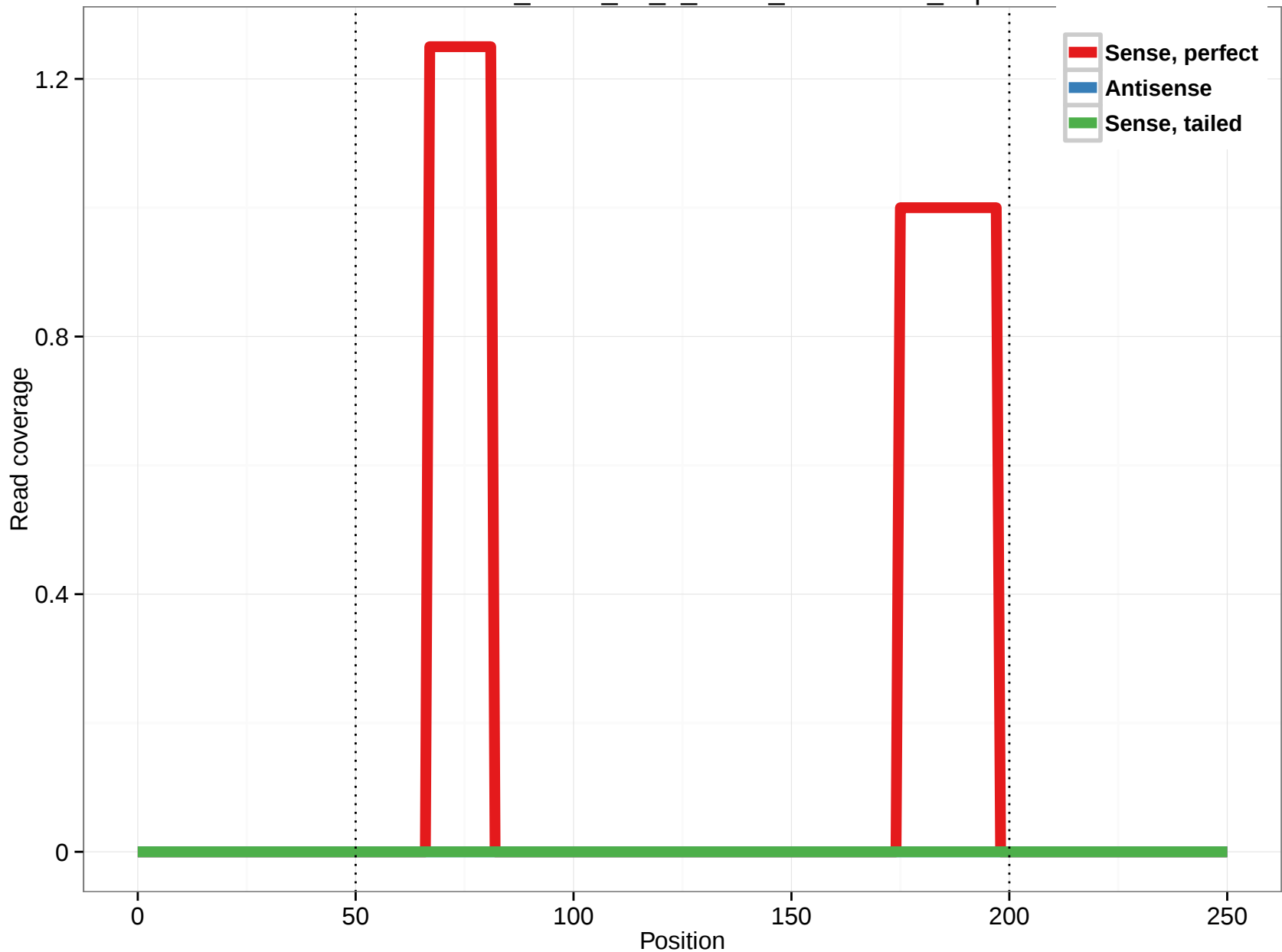
uc010rxk.1_intron_10_0_chr11_117252585_f.3p
