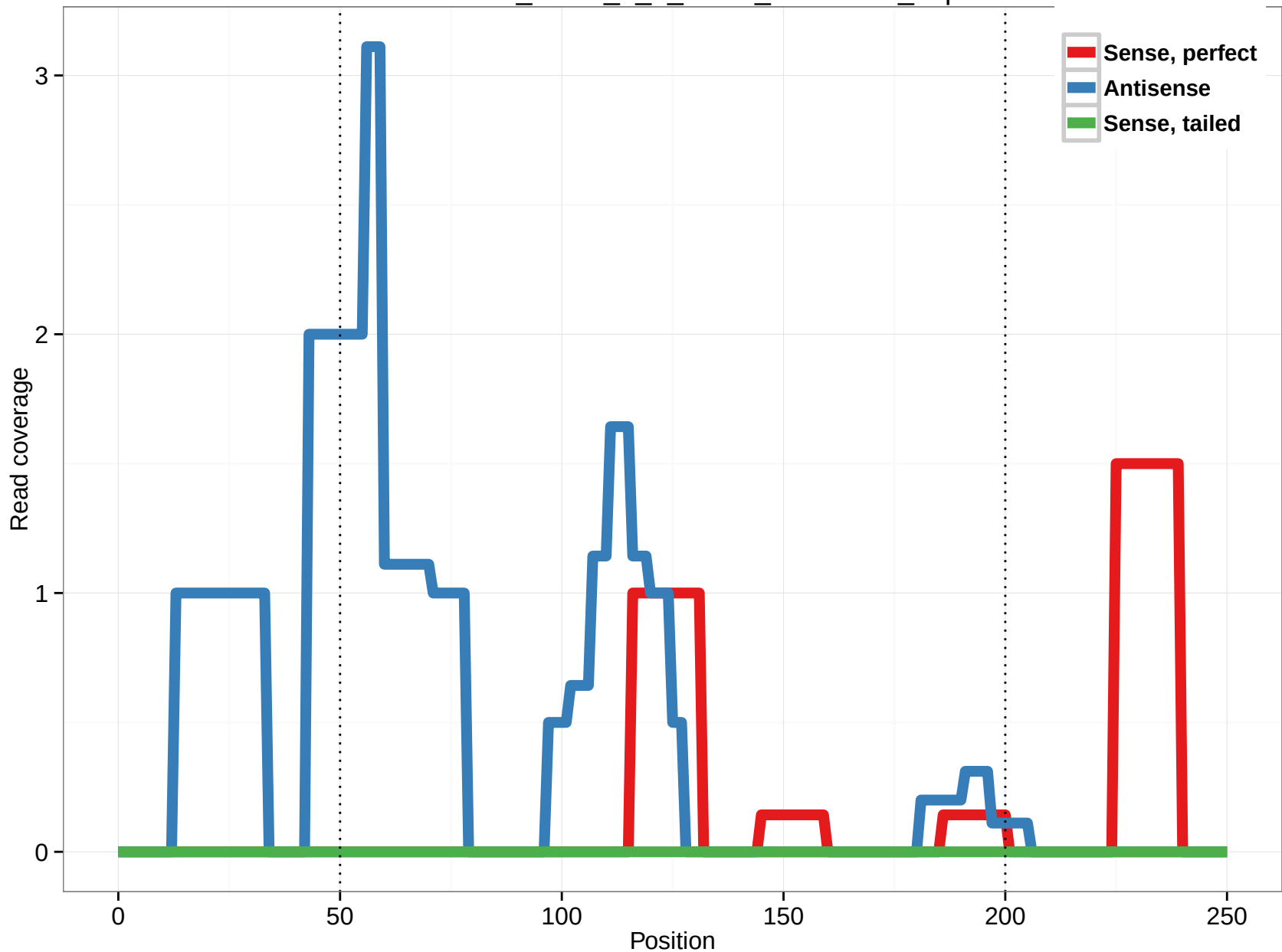
uc010rsl.1_intron_3_0_chr11_76858997_f.5p
