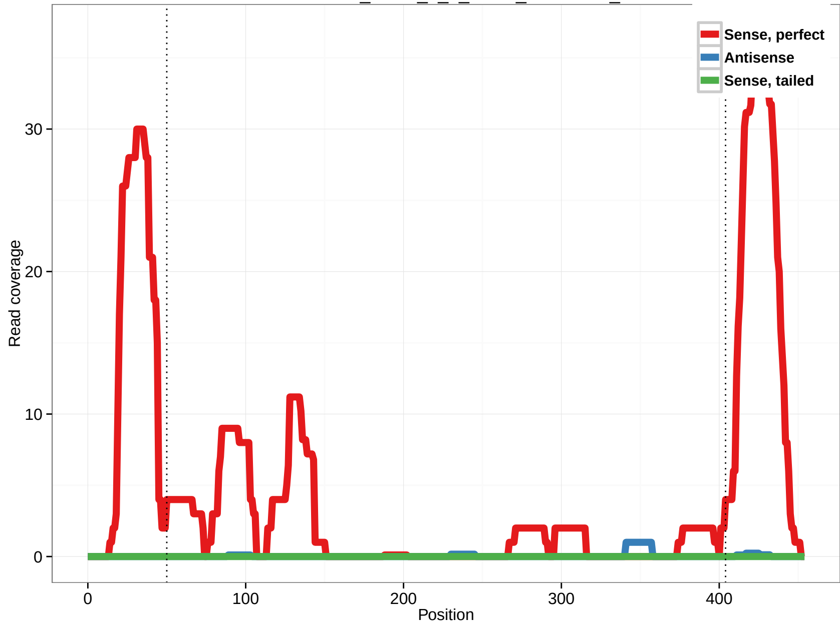
uc010rnn.1_intron_7_0_chr11_64537082_r
