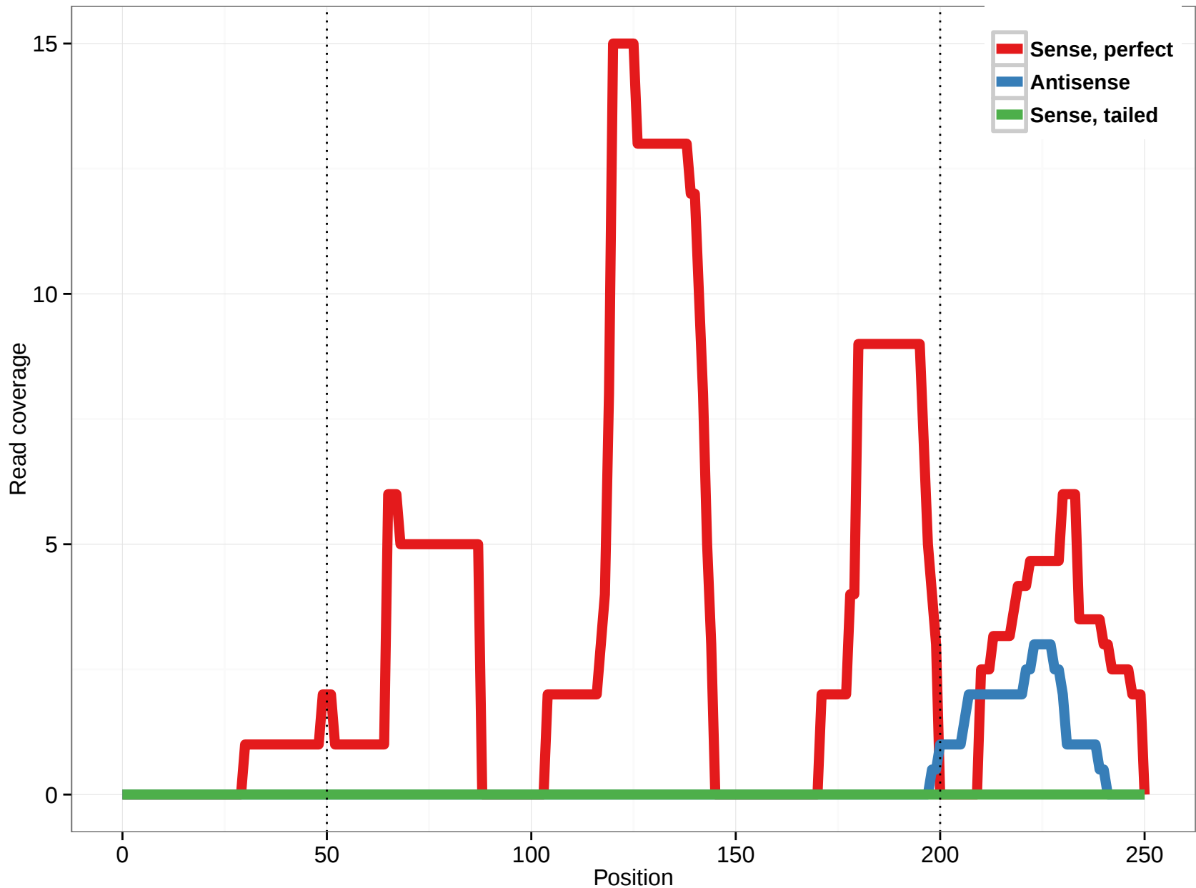
uc010rea.1
