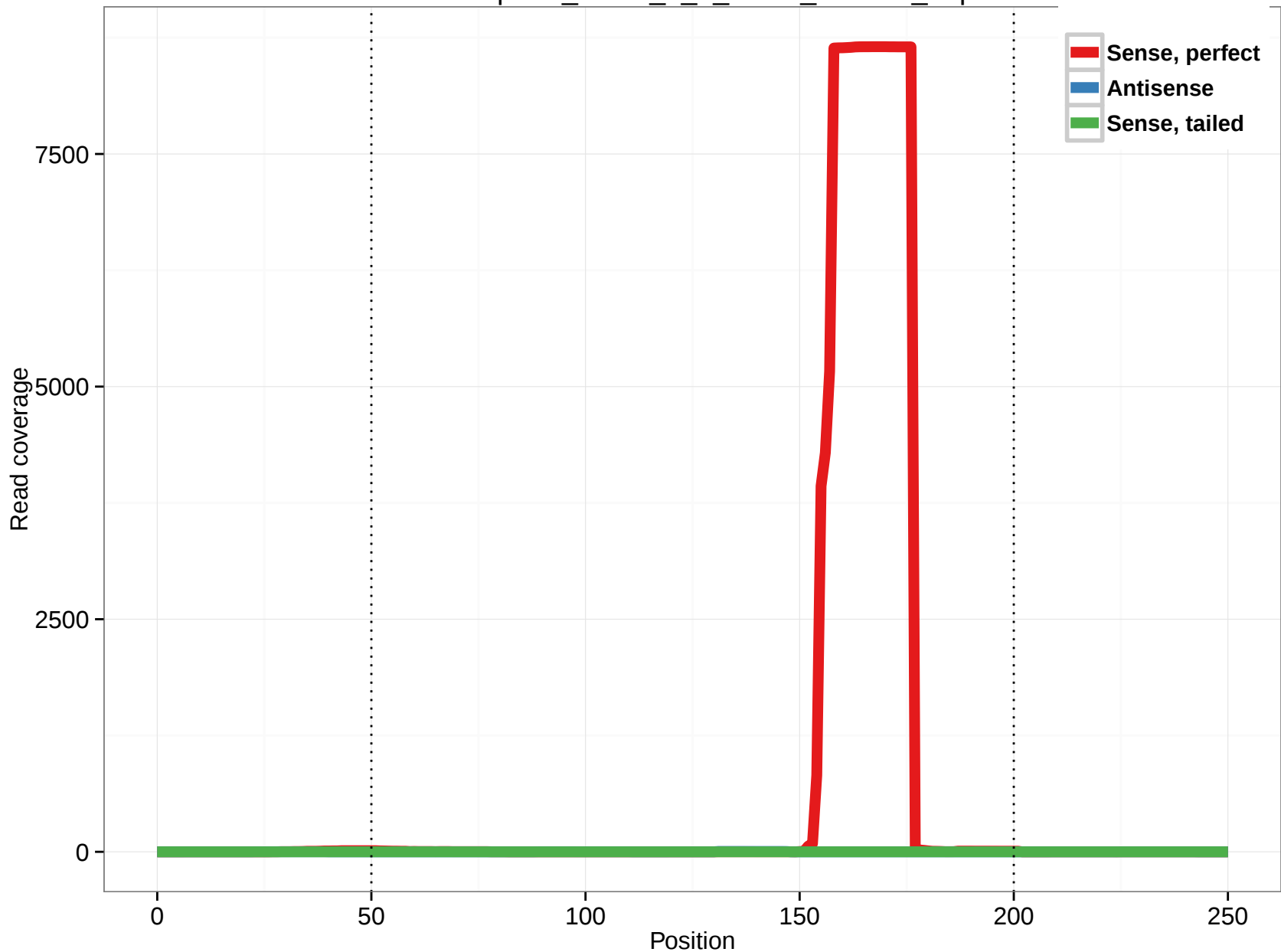
uc010qvw.1_intron_4_0_chr11_534376_r.5p
