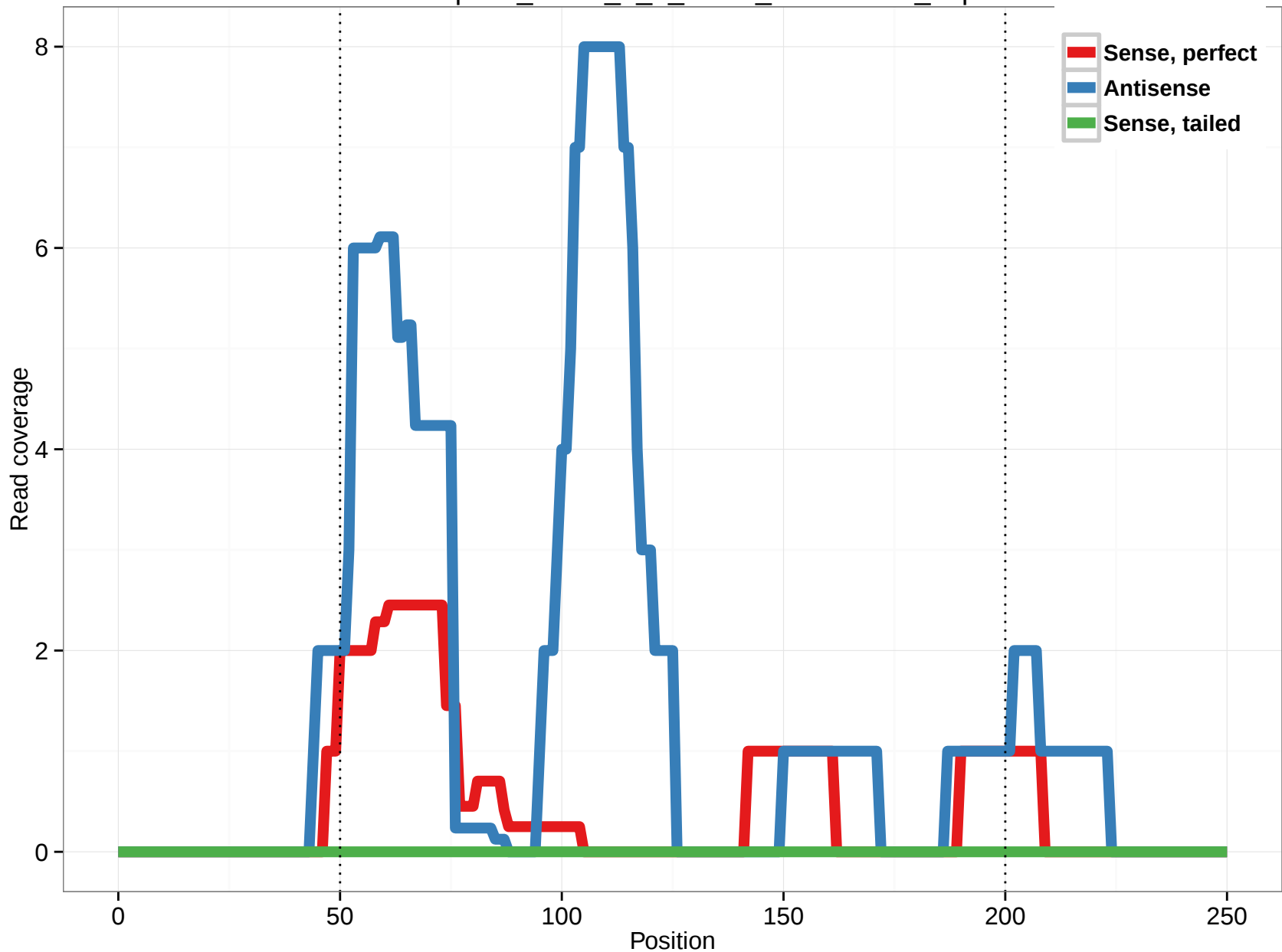
uc010qua.1_intron_2_0_chr10_124641184_f.3p
