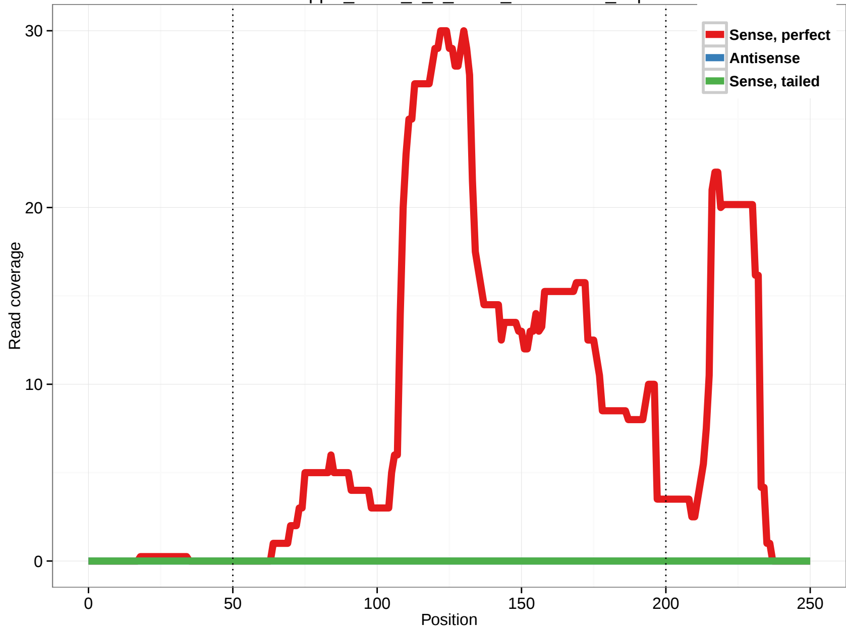
uc010qqf.1_intron_2_0_chr10_103569974_r.3p
