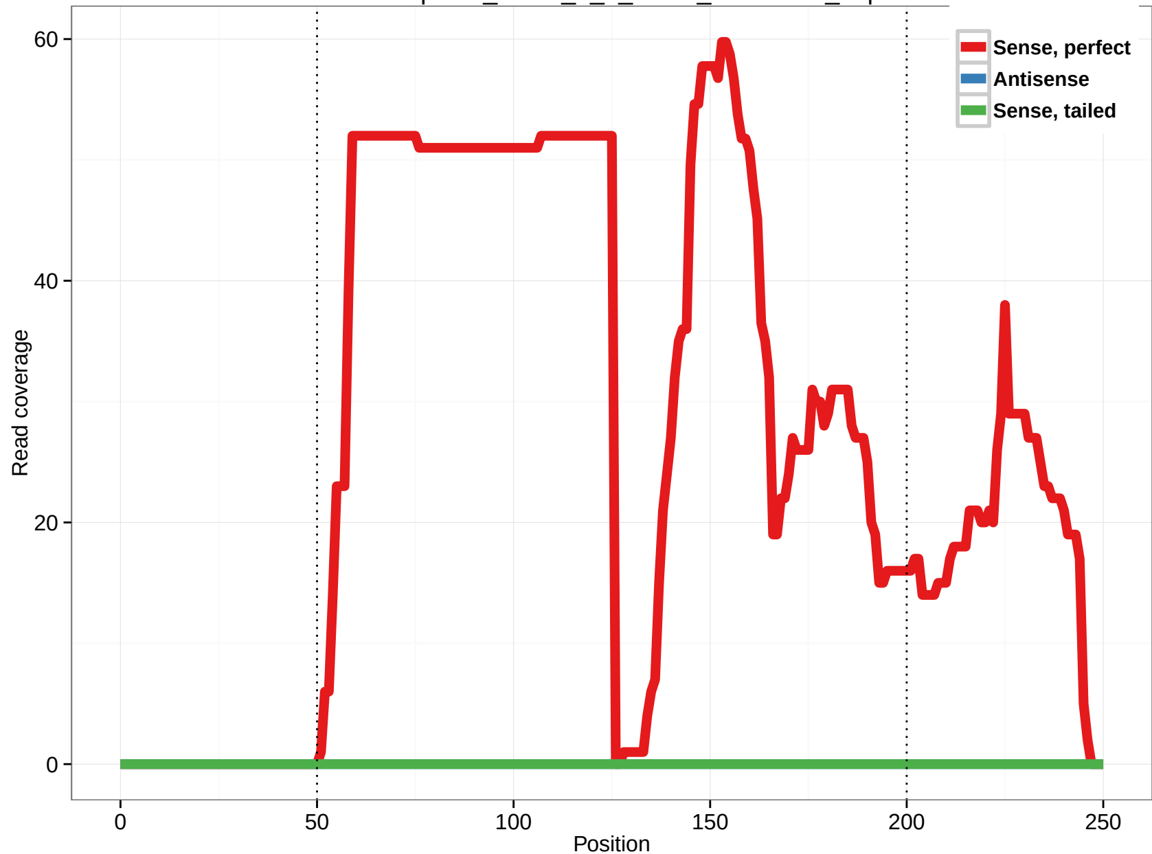
uc010qma.1_intron_3_0_chr10_85903863_f.3p
