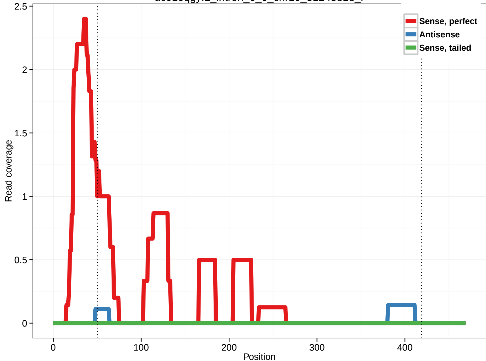
uc010qgy.1_intron_6_0_chr10_51245818_r
