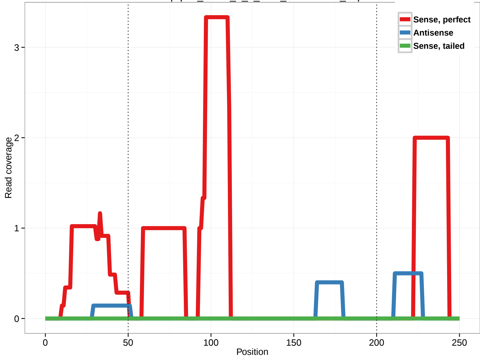
uc010pqn.1_intron_3_0_chr1_203834248_f.5p
