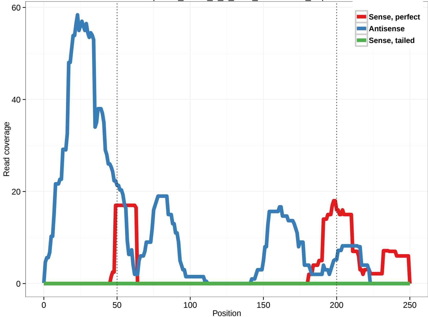
uc010pow.1_intron_9_0_chr1_193020948_r.5p
