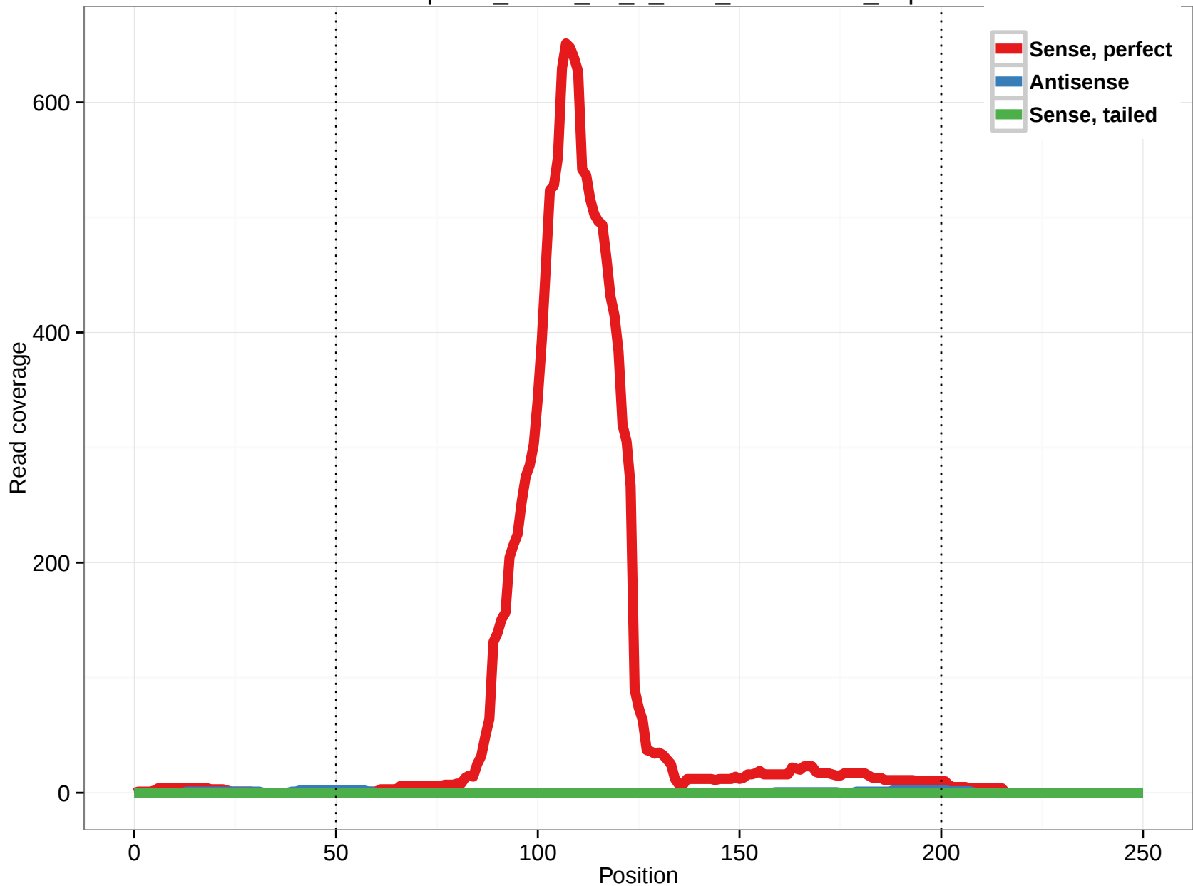
uc010pon.1_intron_13_0_chr1_185121068_r.5p
