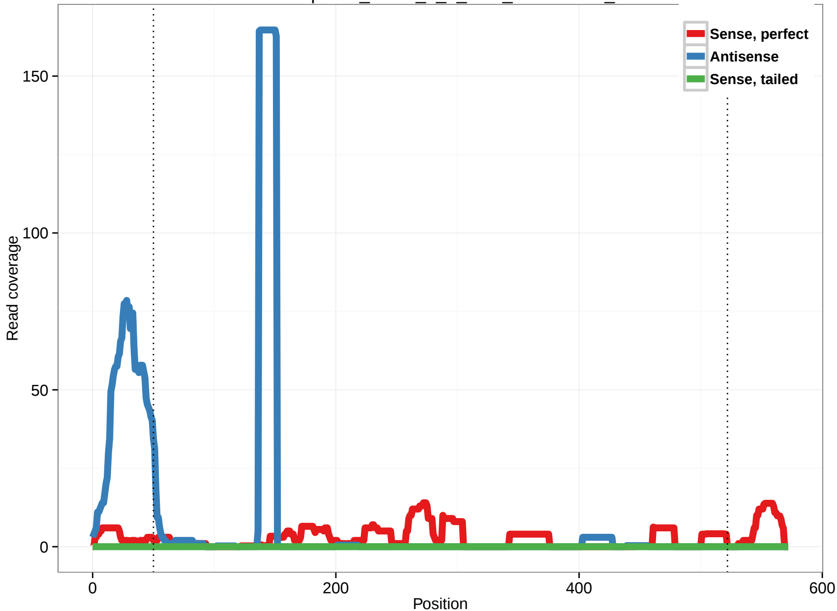
uc010pew.1_intron_1_0_chr1_155057881_f
