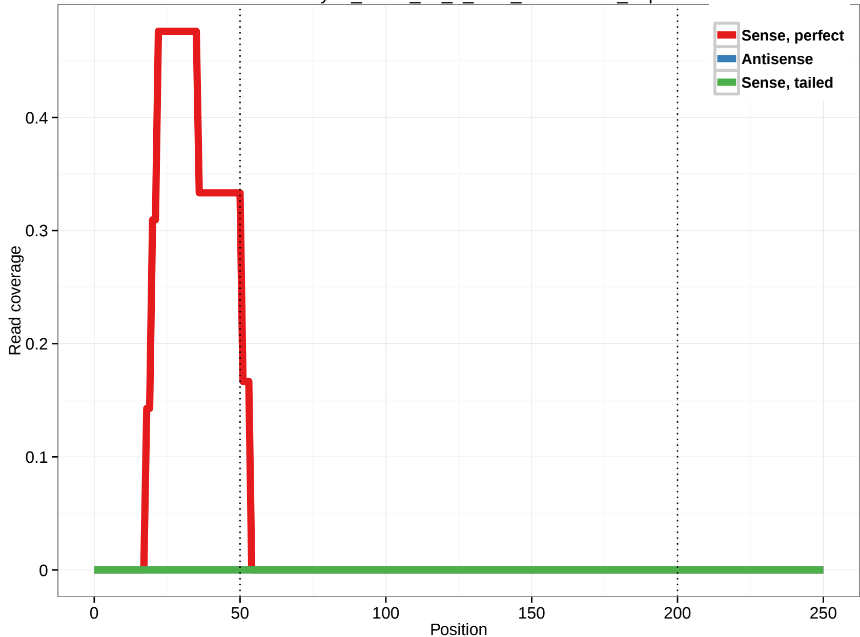
uc010oyr.1_intron_18_0_chr1_145362270_f.3p
