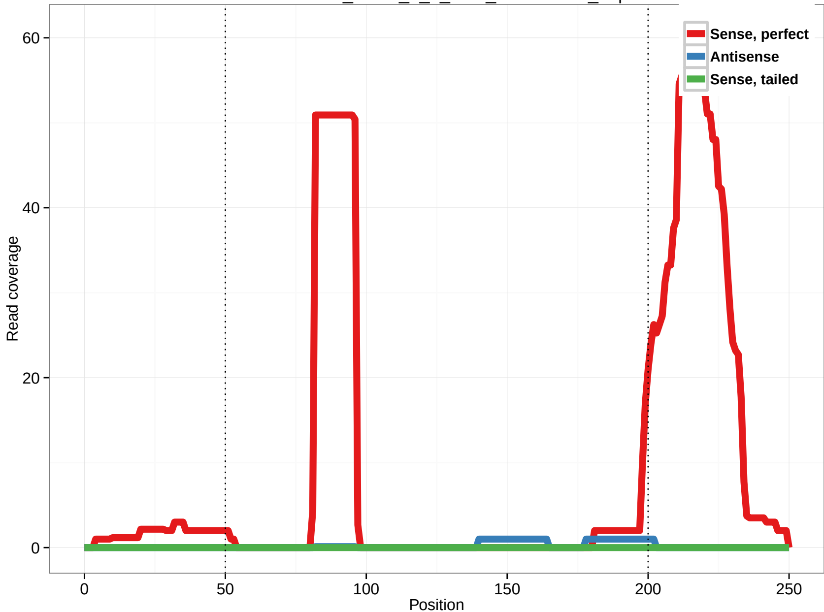
uc010owv.1_intron_9_0_chr1_116933514_f.3p
