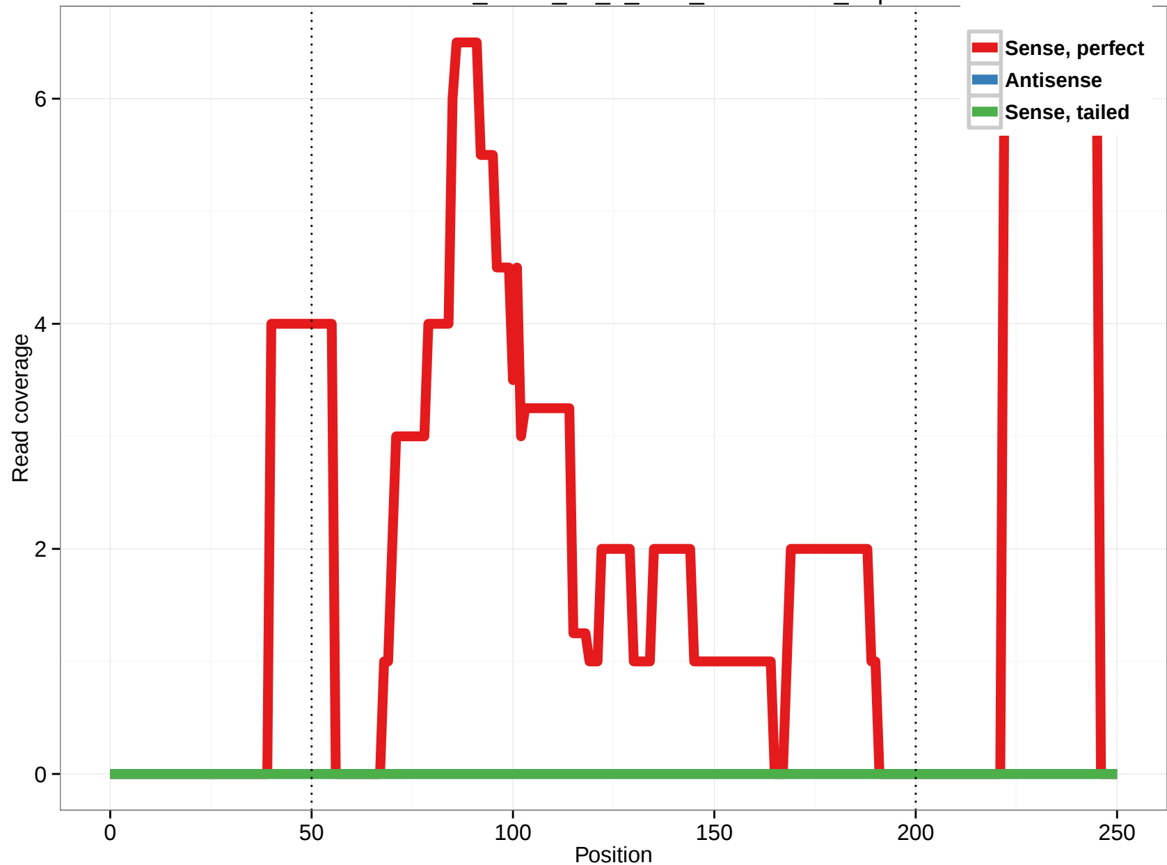
uc010ows.1_intron_12_0_chr1_114968346_r.3p
