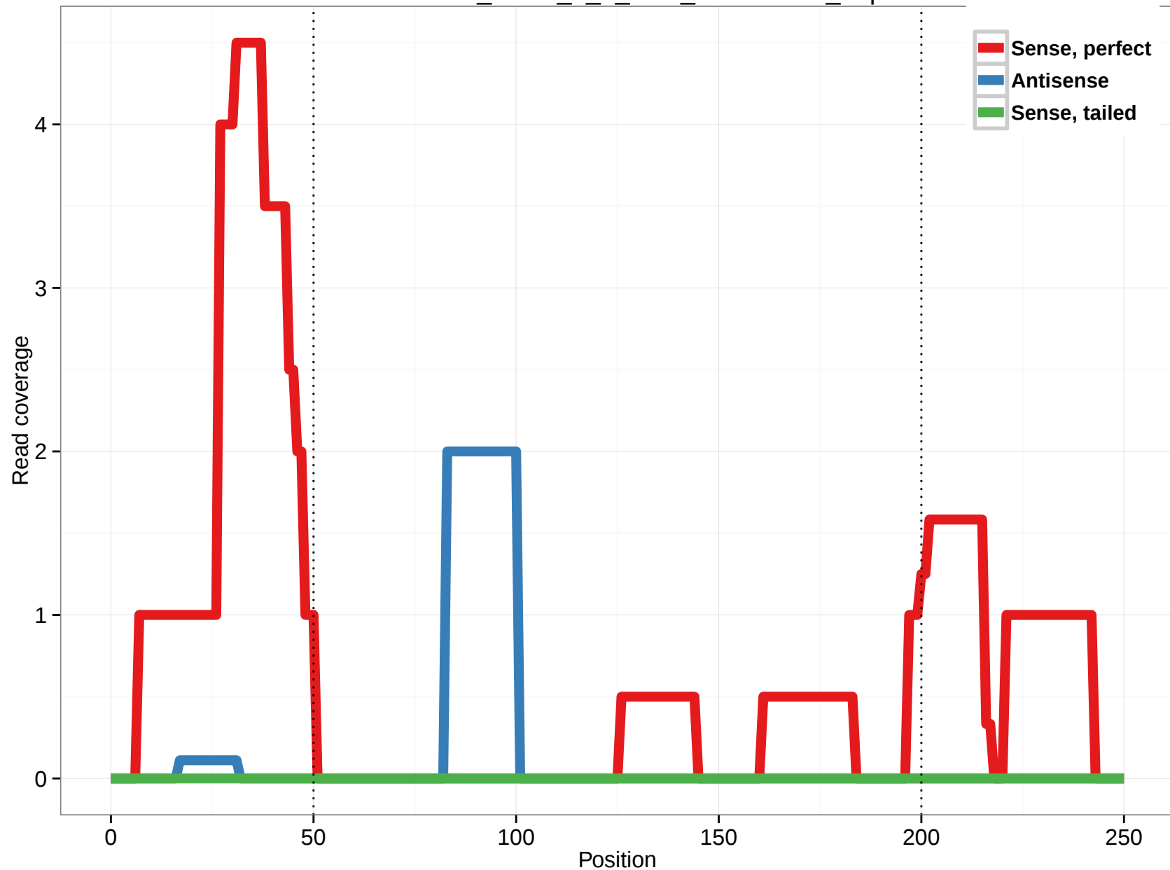
uc010ovf.1_intron_5_0_chr1_109529303_r.5p
