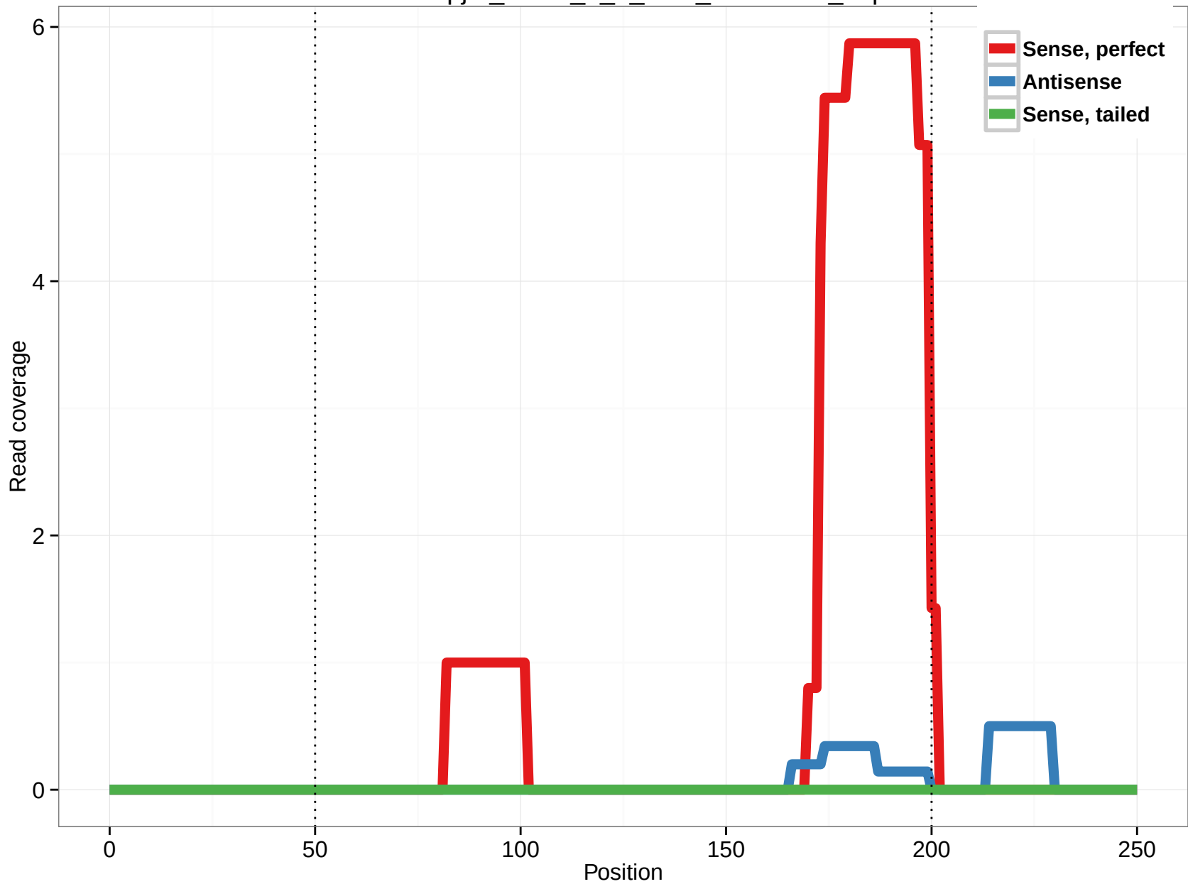
uc010opj.1_intron_1_0_chr1_67648643_f.3p
