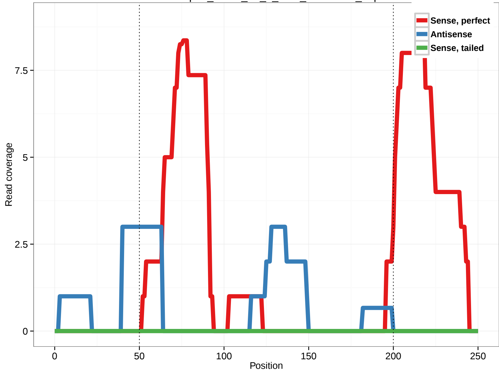
uc010opf.1_intron_12_0_chr1_67442406_f.3p
