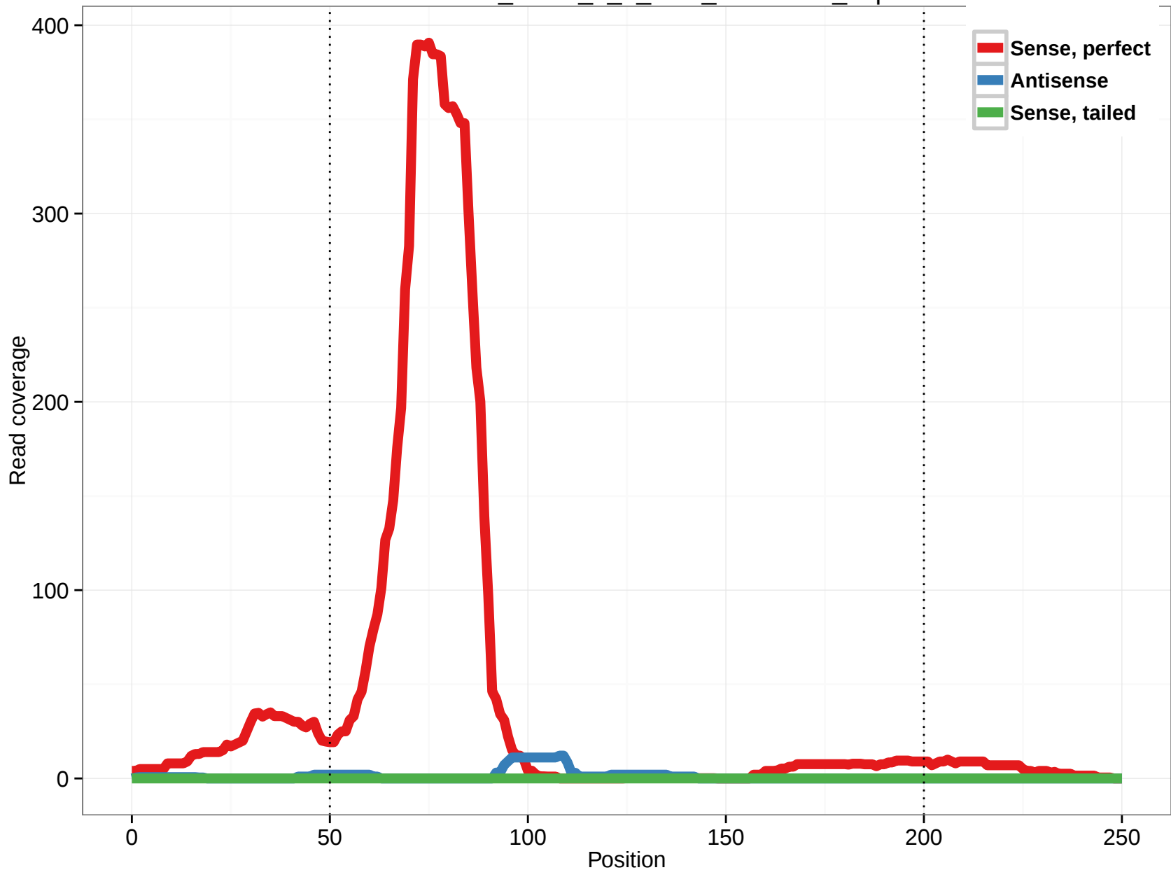
uc010oos.1_intron_0_0_chr1_61547720_f.3p
