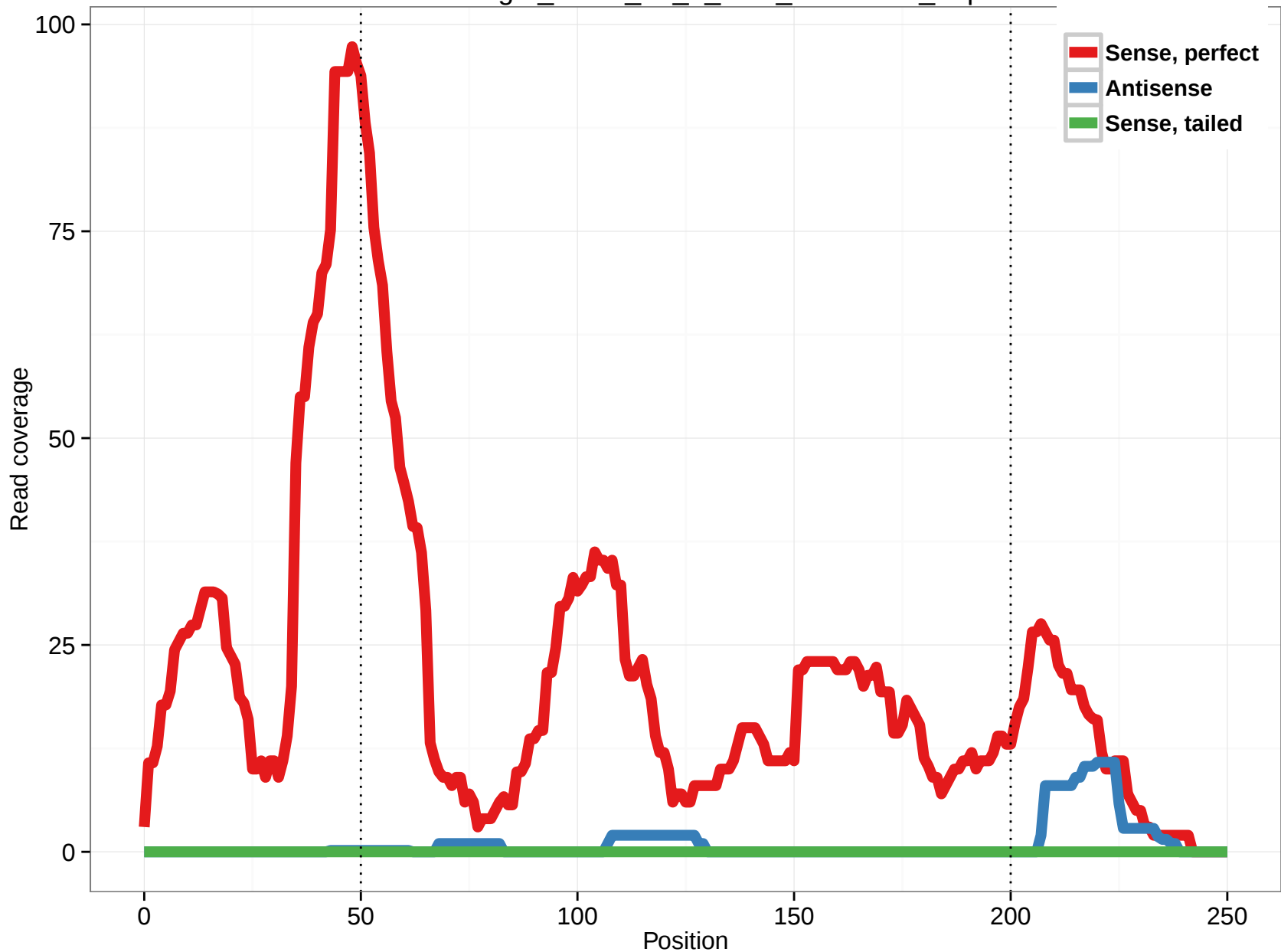
uc010ong.1_intron_23_0_chr1_52306187_r.5p
