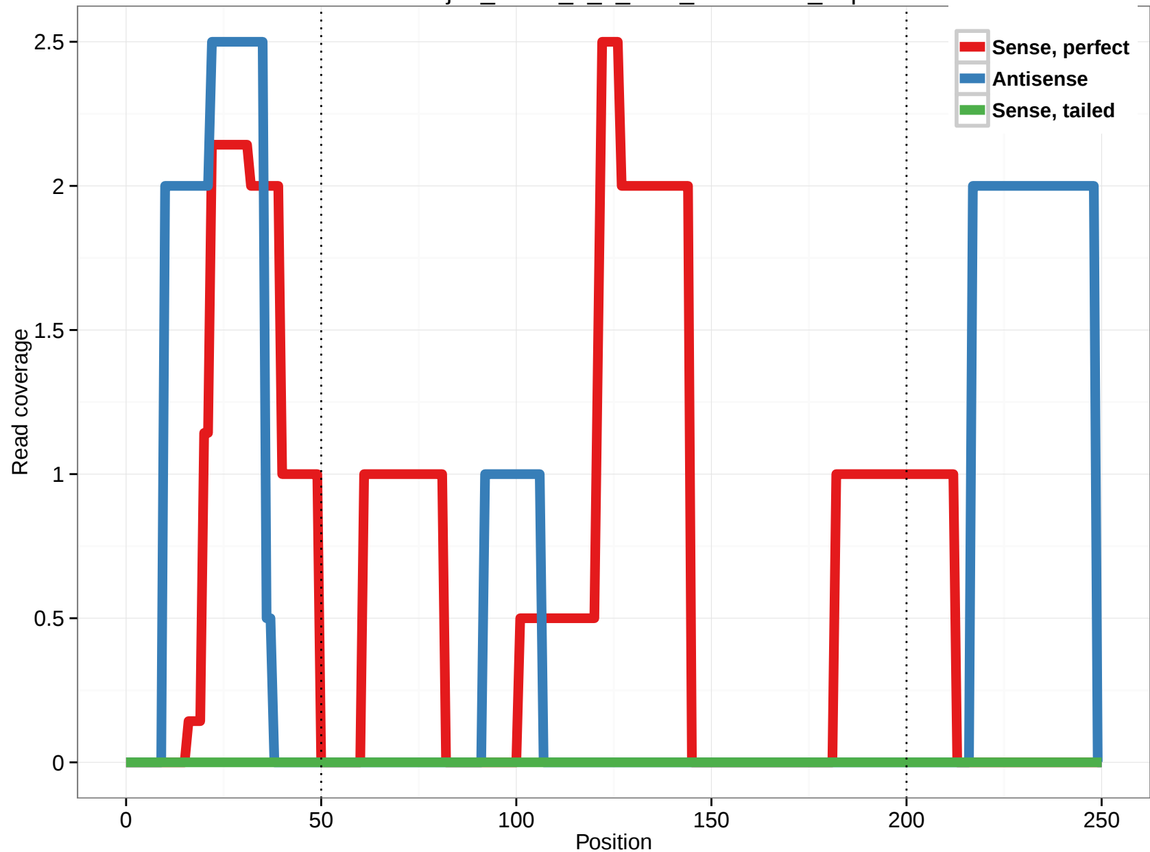
uc010ojr.1_intron_5_0_chr1_41536394_r.5p
