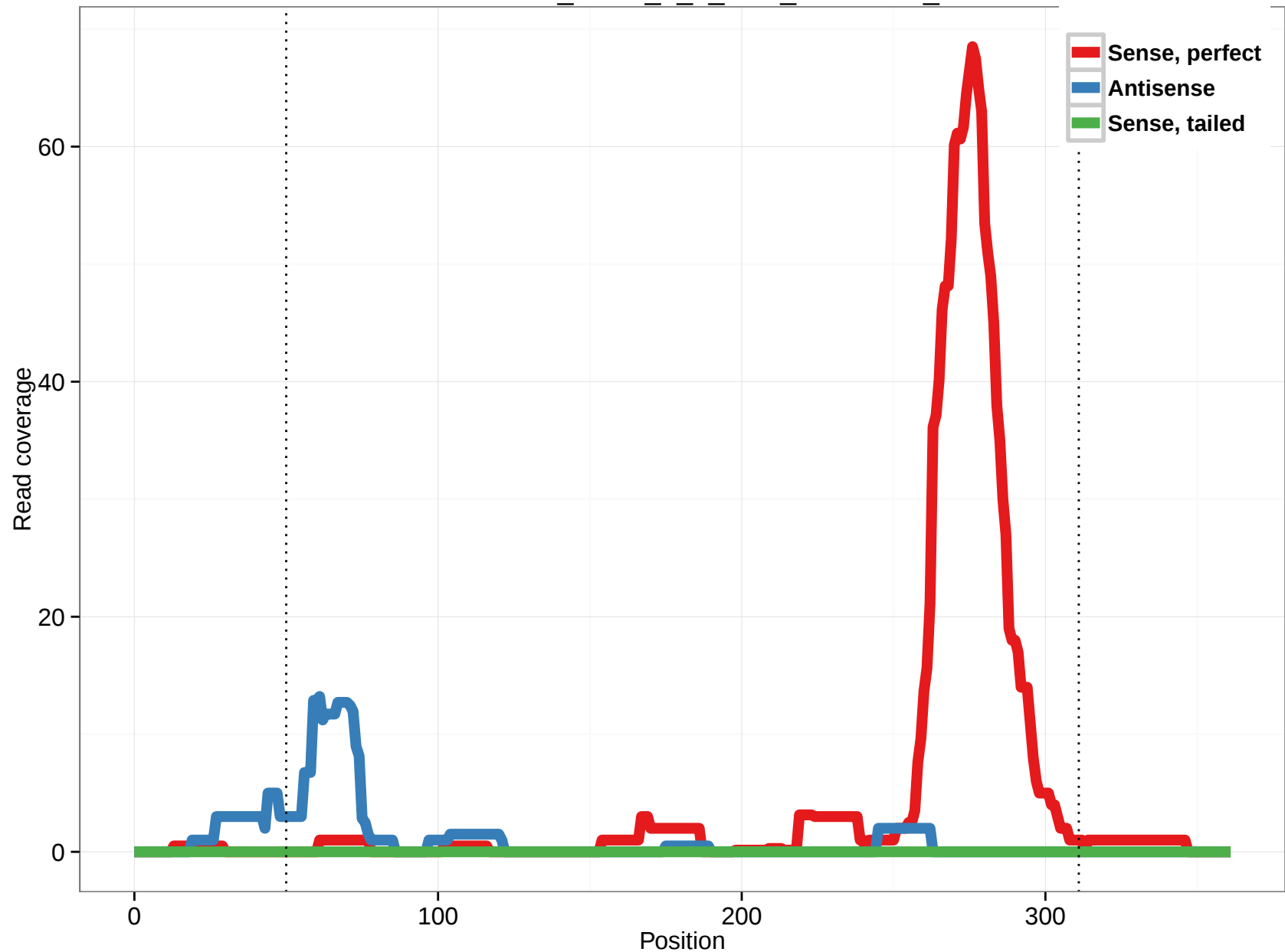
uc010oia.1_intron_2_0_chr1_36772507_f
